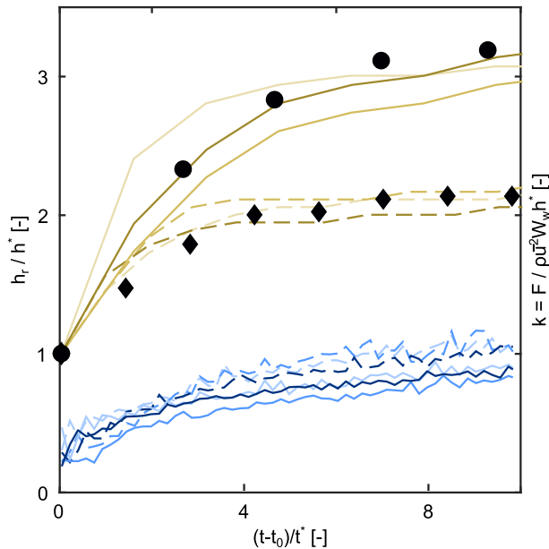
Fig. 9. Comparison of experimental and numerical results for run-up height h_r . The experimental data for run-up at \theta = 28^\circ (diamonds) and \theta = 30^\circ (circles) are displayed alongside the numerical results for both slope angles. Additionally, the dimensionless force coefficient k is included for both slope angles. The time is scaled using the time of first impact t_0 and the reference timescale t^* .
