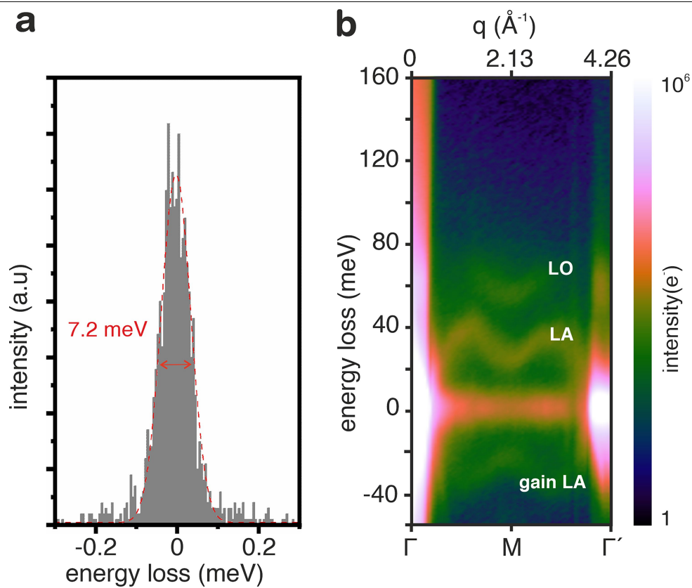
Extended Data Fig. 2 | Vibrational EELS measurements of NiO. a. EELS spectrum corresponding to a single acquisition frame (75 ms) in vacuum, showing a ZLP measuring 7.2 meV at the FWHM. b. As-acquired \omega - q maps along
