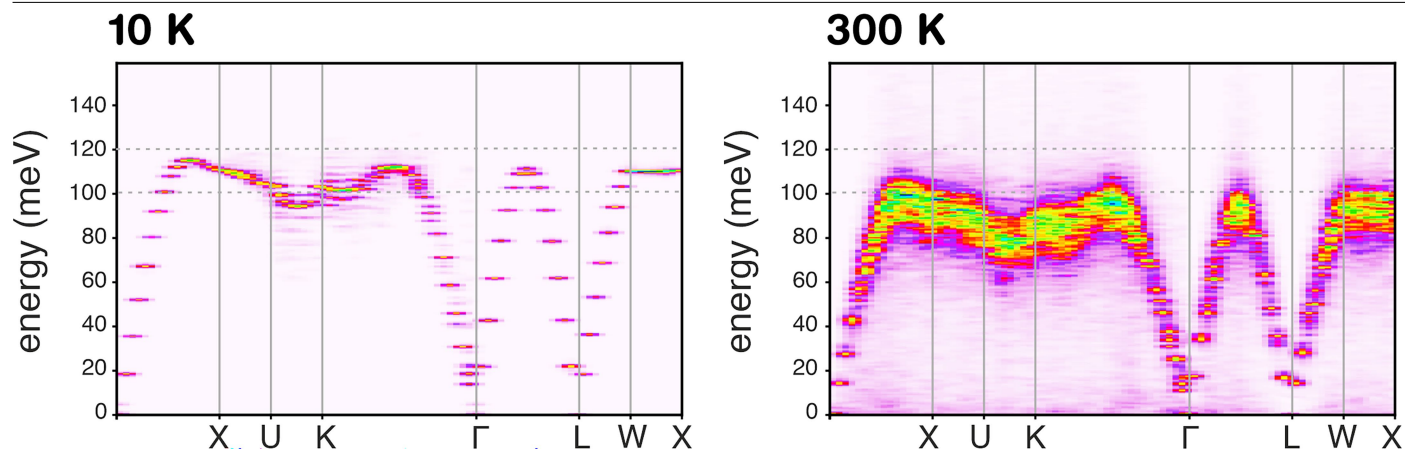
Extended Data Fig. 3 | Magnon dispersions at different temperatures. Calculated magnon dispersions corresponding to the dynamical structure factor computed using UppASD 34 for a NiO supercell consisting of 32 \times 32 \times 32 repetitions of the cubic unit cell with periodic boundary conditions applied in
