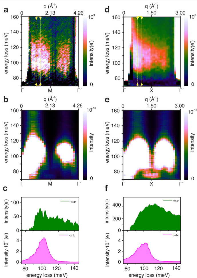
Extended Data Fig. 4 | Experiment versus theory. a,b,d,e , Experimental background-subtracted ( a,d ) and calculated ( b,e ) \omega - q EELS maps showing the dispersion of the magnon bands above 100 meV. c,f , Extracted spectra over a narrow momentum window ( \Delta q = 0.22 \text{ \AA}^{-1} ), to avoid spectral broadening through momentum averaging, at the value at which the intensity is maximum along \Gamma \rightarrow M ( q = 1.24 \text{ \AA}^{-1} ) and \Gamma \rightarrow X ( q = 0.97 \text{ \AA}^{-1} ), marked by the yellow arrows and dashed lines in a and d , respectively. Calculated spectra at the same wave vector and averaged over a similar momentum window highlight the shape of the peaks, with a rising edge from 80 meV reaching a maximum at about 100 meV, before a weaker feature extending up to 120 meV, with the peak observed along \Gamma \rightarrow X being broader and more rounded.
