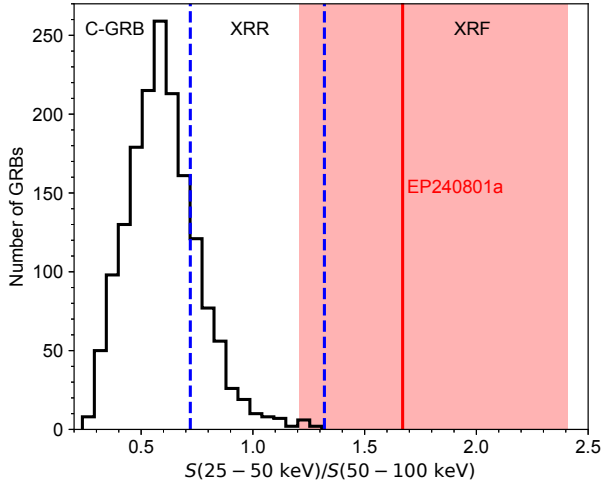
Figure 6. The fluence ratio S(25\text{--}50\text{ keV})/S(50\text{--}100\text{ keV}) of 1647 GRBs recorded in the Fermi/GBM archive from 2008 to 2020; most of them are C-GRBs due to the higher trigger threshold of Fermi/GBM for the soft events. The red line represents the fluence ratio of EP240801a, and the shadow is the 1\sigma uncertainty interval. The blue dashed lines represent the boundaries of C-GRBs, XRRs, and XRFs described by T. Sakamoto et al. (2008).
