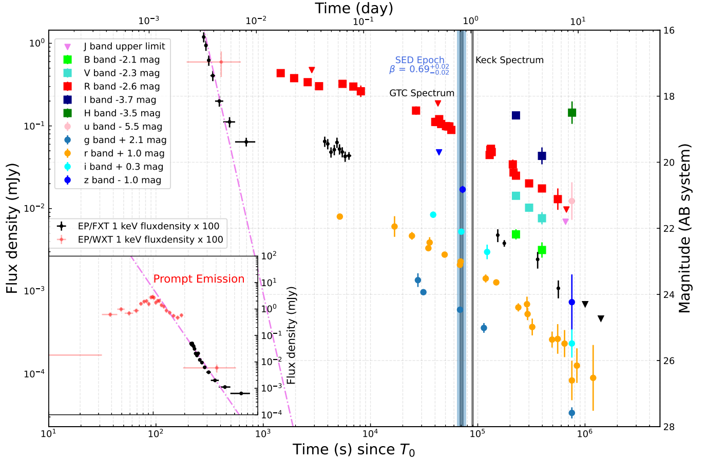
Figure 7. Light curves of EP240801a from the prompt phase to the afterglow phase in X-rays, optical, and NIR. The EP/WXT (red circles) and EP/FXT (black circles) data are presented with unabsorbed flux density at 1 keV and scaled by a factor of 100 in the main figure but not scaled in the inset. The inset shares the time axis with the main figure. The optical/NIR data are in the AB system (J. B. Oke & J. E. Gunn 1983) and have been corrected for Galactic extinction, which is E(B - V) = 0.093 mag (E. F. Schlafly & D. P. Finkbeiner 2011), and the host-galaxy magnitude. All the inverted triangle symbols signify limits. The light blue slice represents the time of the SED. Two gray slices represent the time of the GTC and the Keck optical spectrum, respectively. A violet dashed-dotted single power law with \alpha = 5.82 \pm 0.32 is depicted in both the main figure and the inset.
