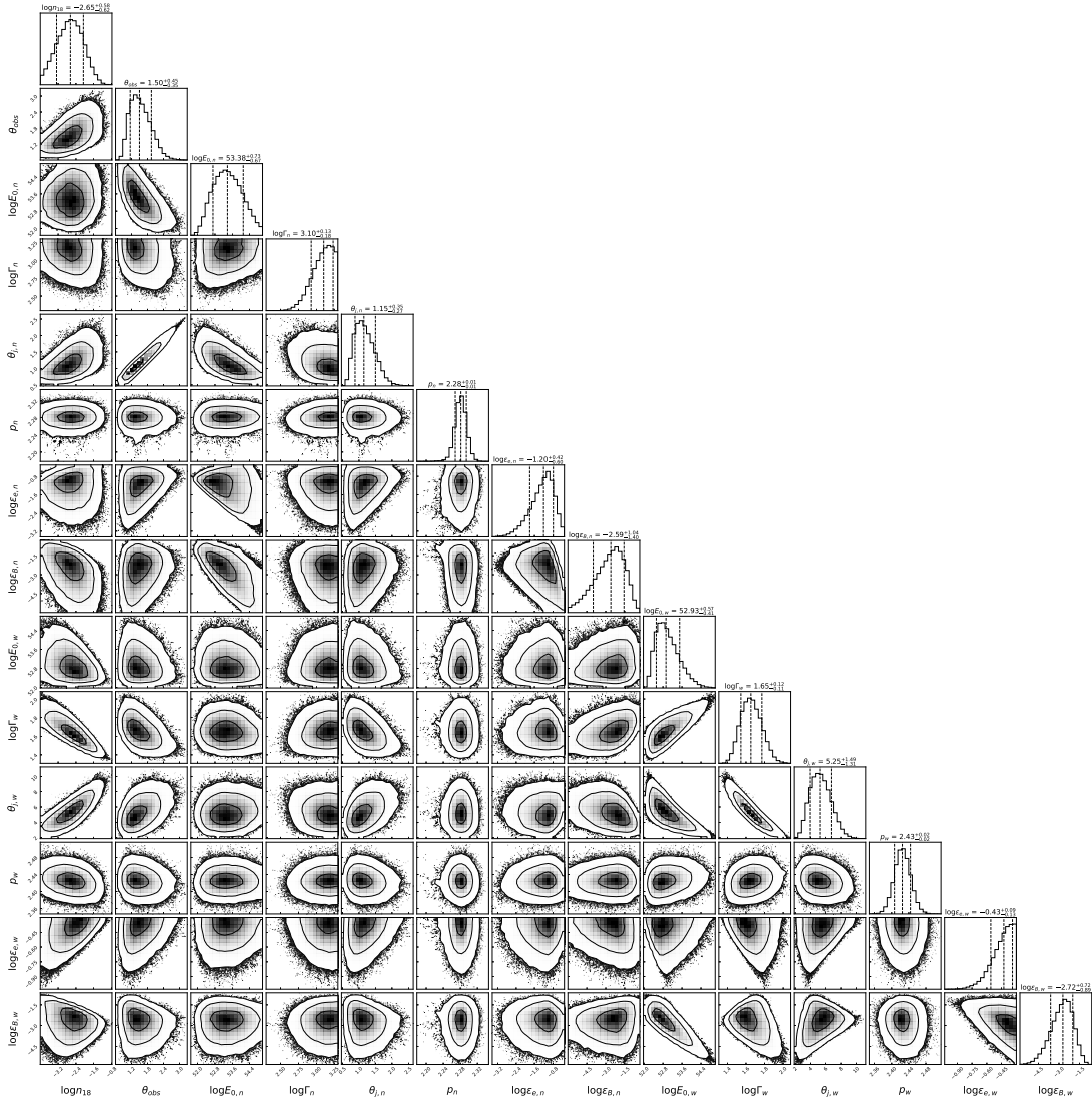
Figure D1. Posterior probability distributions of the afterglow parameters were obtained using the two-component jet modeling of EP240801a. The median values with the 1\sigma regions are shown in the 1D probability distribution.
