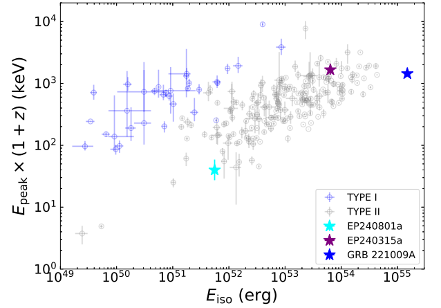
Figure 5. Amati diagram of EP240801a (cyan star); the blue and gray circles represent other type I and type II GRBs, respectively. Another GRB detected by EP, EP240315a, is marked as a purple star. GRB 221009A is marked as a blue star.
