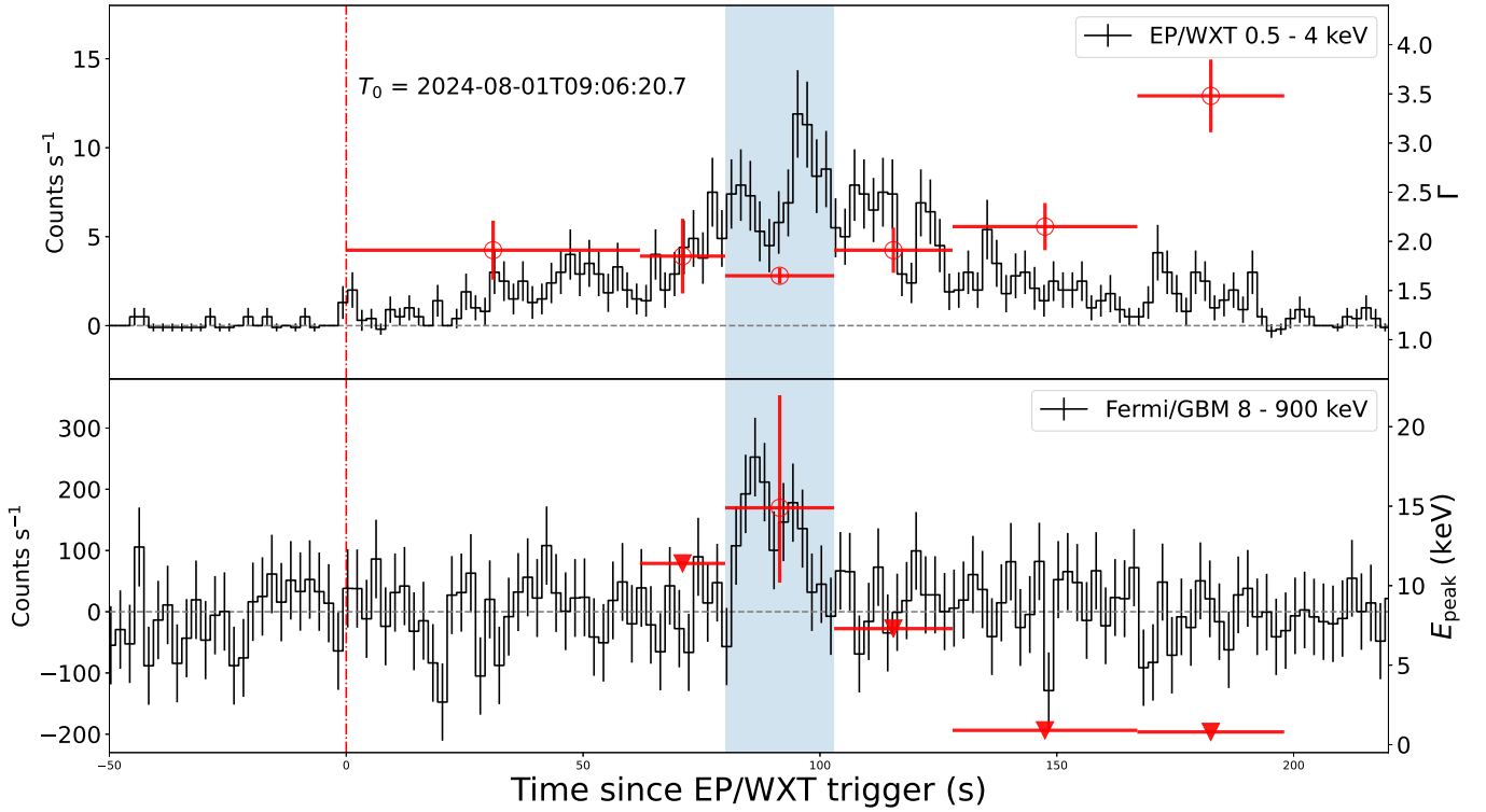
Figure 1. The prompt emission light curve obtained by EP/WXT and Fermi/GBM; the gray dotted lines indicate zero count rate. The red dashed-dotted line represents the T_0 of EP240801a, and the UTC time is indicated. We analyzed the joint spectrum of EP/WXT and Fermi/GBM data during the vertical light blue slice. The photon index (red circles) of the time-resolved fit of the EP/WXT data is shown in the upper panel. The lower panel depicts the E_{\text{peak}} of EP240801a, and the inverted triangle symbols signify limits.
