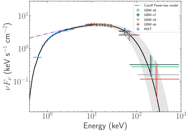
Figure 4. The spectral joint fitting of EP/WXT and Fermi/GBM data during the light blue slice in Figure 1. The black solid line represents the best-fit absorbed cutoff power-law model, and the shadow is the 1\sigma uncertainty interval, while the violet dashed-dotted line shows the individual cutoff power-law model. The data from different detectors are marked as various colors.
