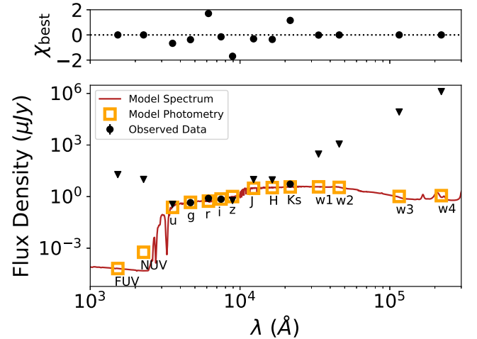
Figure 9. SED of the host galaxy of EP240801a. The best-fit model SED is shown by the red line. \chi_{\text{best}} means a standardized residual. The model photometry results are marked as squares with their corresponding bands below, and the observed data are indicated by black data points (black inverted triangles represent upper limits). All the data are corrected for Galactic extinction.
