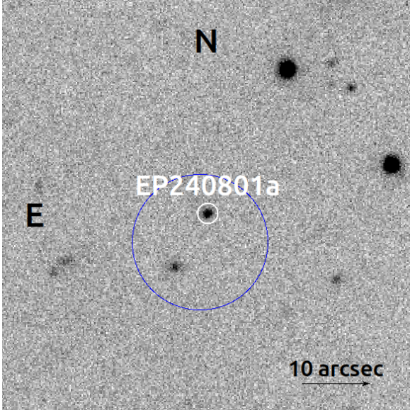
Figure 2. The Sloan r' -band position of EP240801a with the field of view of l' \times l' obtained by NOT/ALFOSC about 0.8 days after the discovery of EP240801a. The location of the burst is circled in white, and the 10'' error circle of EP/FXT is in blue.
