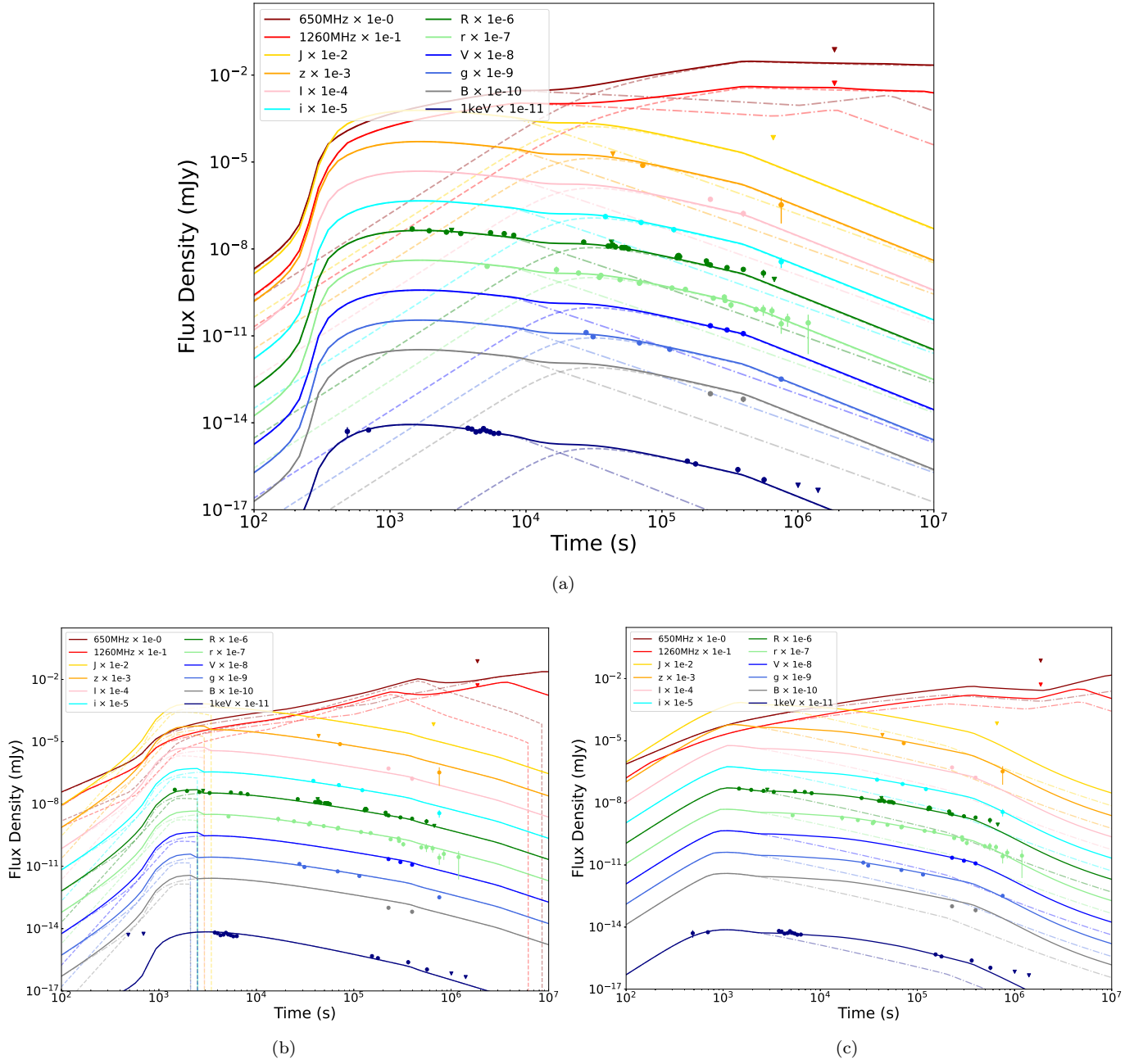
Figure 10. Best-fit results using the PyFRS code with three models (solid lines). (a) A two-component jet model, containing a narrow, faster jet (dashed-dotted lines) as well as a broad, slower jet (dashed lines). (b) FS-RS model. The contributions from the RS and FS are plotted with dashed lines and dashed-dotted lines, respectively. (c) FS with energy injection (solid lines). The FS without energy injection is represented by the dashed-dotted lines.
