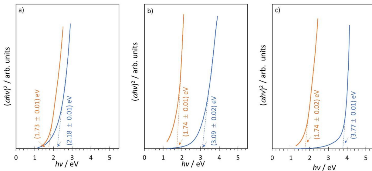
Fig. 14 (\alpha h\nu)^2 vs. h\nu dependence of (a) QD-75, (b) QD-55 and (c) QD-75US unannealed (blue) and annealed at 200 °C for 2 h (orange), respectively.
