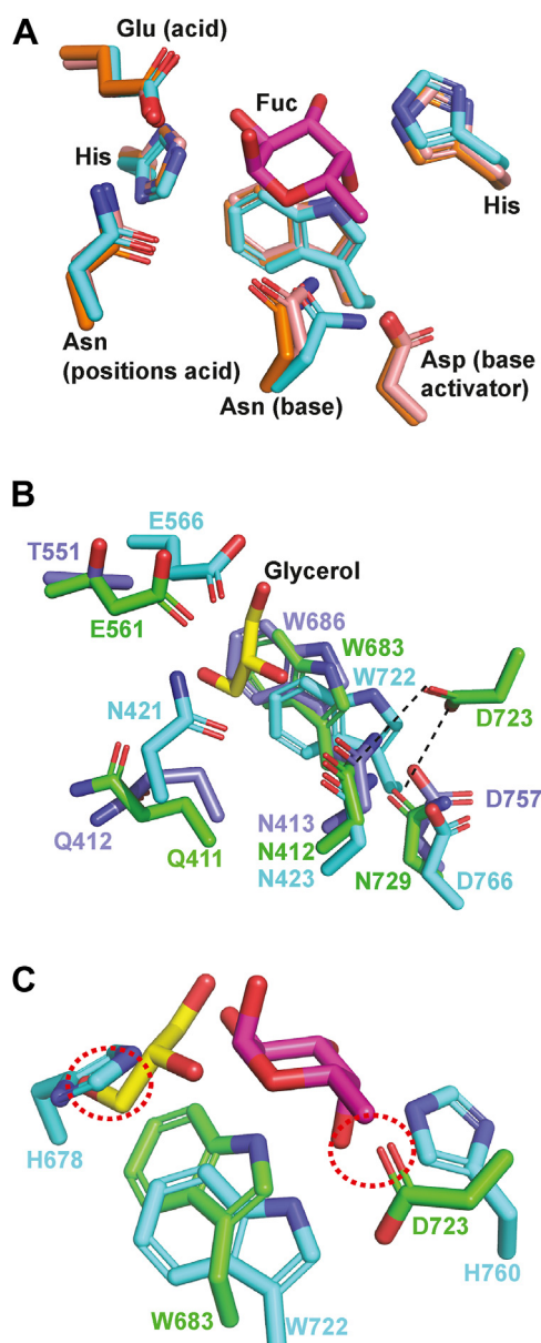
Figure 4. Architecture of the –1 subsite distinguishes GH139 enzymes from GH95 \alpha -L-fucosidases. A, close-up views of the –1 subsite of three representative GH95s: PDB codes: 2EAE (cyan), 4UFC (pink), 7KMQ (orange). B, overlay of the –1 subsite of BT0984 GH139 (green), SDT91673.1 GH139 (slate blue), and AfcA GH95 (cyan). The glycerol (yellow) is from the cryoprotectant of SDT91673.1 GH139 . C, overlay of BT0984 GH139 (green) with AfcA GH95 (PDB: 2EAE) (cyan) with L-fucose (PDB: 2EAE) (magenta) illustrating steric clashes introduced by GH139 residues (circled, red) that reshape the pocket and alter substrate specificity.
