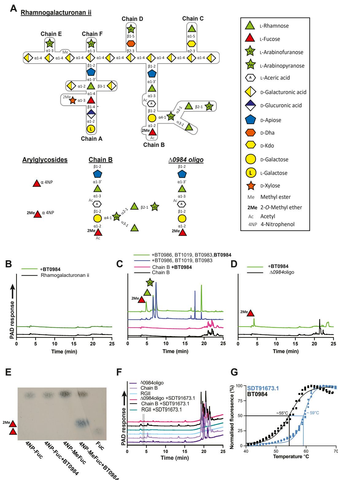
Figure 1. GH139 enzymes cleave RG-II glycans: substrate structures, activity and thermal stability. A, structure of rhamnogalacturonan ii and fragment glycan substrates used in this study; (B) high-performance anion exchange chromatography (HPAEC) of BT0984 GH139 against rhamnogalacturonan ii; (C) HPAEC of BT0984 GH139 against isolated chain B; (D) HPAEC of BT0984 GH139 against \Delta 0984 oligo; (E) thin layer chromatography of BT0984 GH139 versus 4NP- \alpha -L-fucopyranoside and 4NP- \alpha -L-2-O-methylfucopyranoside; (F) HPAEC of SDT91673.1 GH139 versus rhamnogalacturonan ii, isolated chain B, and \Delta 0984 oligo; the grey box indicates the expected position of 2-O-methylfucose and shows it is absent. Enzyme concentrations used were 1 \mu M in 10 mM MOPS buffer pH 7.0 with 150 mM NaCl. G, DSF analysis of GH139 stability.
