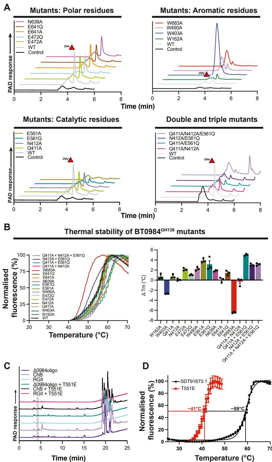
Figure 7. Catalytic-site mutations alter GH139 activity toward \Delta bt0984 oligo and reduce thermal stability. A, HPAEC-PAD traces from overnight endpoint assays comparing wild-type BT0984 GH139 and its mutant variants (1 \mu M enzyme, 10 mM MOPS pH 7.0, 150 mM NaCl). B, differential scanning fluorimetry of BT0984 GH139 variants. Left: normalized melt curves. Right: bar graph of \Delta T_m mutants versus wildtype. C, HPAEC-PAD analysis of the SDT91673.1 T551E mutant against rhamnogalacturonan ii, isolated chain B, and \Delta 0984oligo; absence of methylfucose release is indicated in the grey window. D, DSF melt curves of SDT91673.1 GH139 wild type versus the T551E variant, highlighting the destabilizing effect of the substitution.
