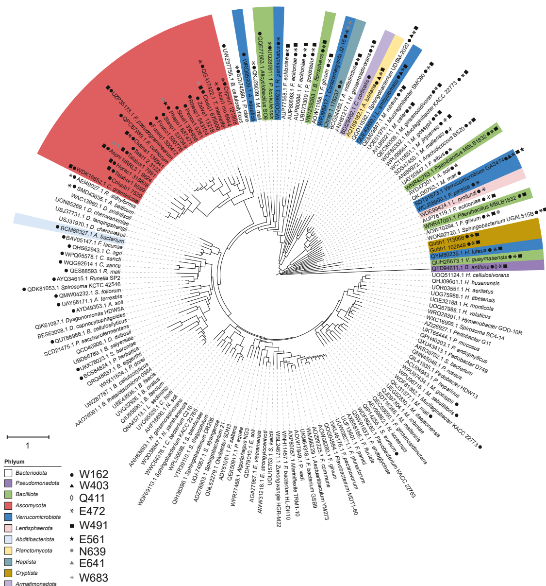
Figure 6. Phylogeny of GH139 enzymes highlights phylum-level clades and divergence of catalytic residues. Unrooted maximum-likelihood tree constructed in MEGA X based on alignment of amino acid sequences of each family member obtained from both NCBI and JGI databases. Branch lengths are proportional to the number of substitutions per site; branches are colour coded by phylum. Symbols indicate the lack of conservation of corresponding key residues in homologues of Bacterioides thetaiotaomicron . Sequence identifiers have been truncated for clarity.
