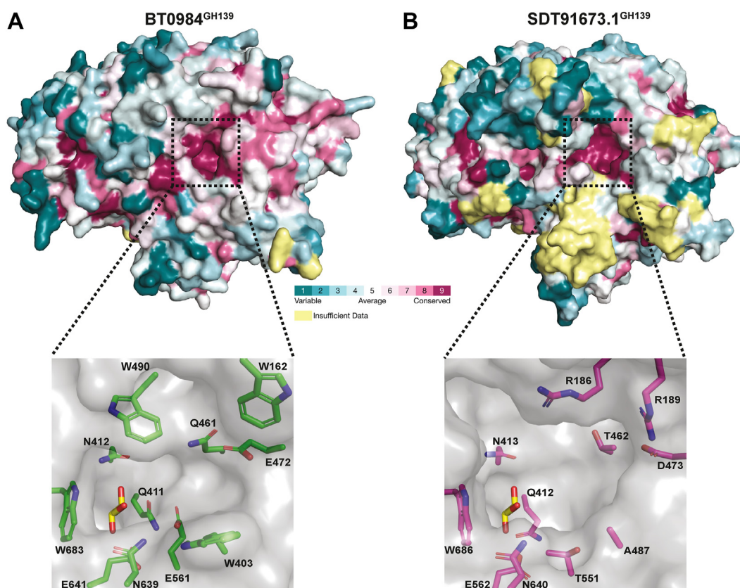
Figure 5. Identification of the active site of family GH139 enzymes. A, consurf analysis of BT0984 GH139 with a zoom in of the putative active site. B, consurf analysis of SDT91673.1 GH139 with a zoom in of the putative active site.
