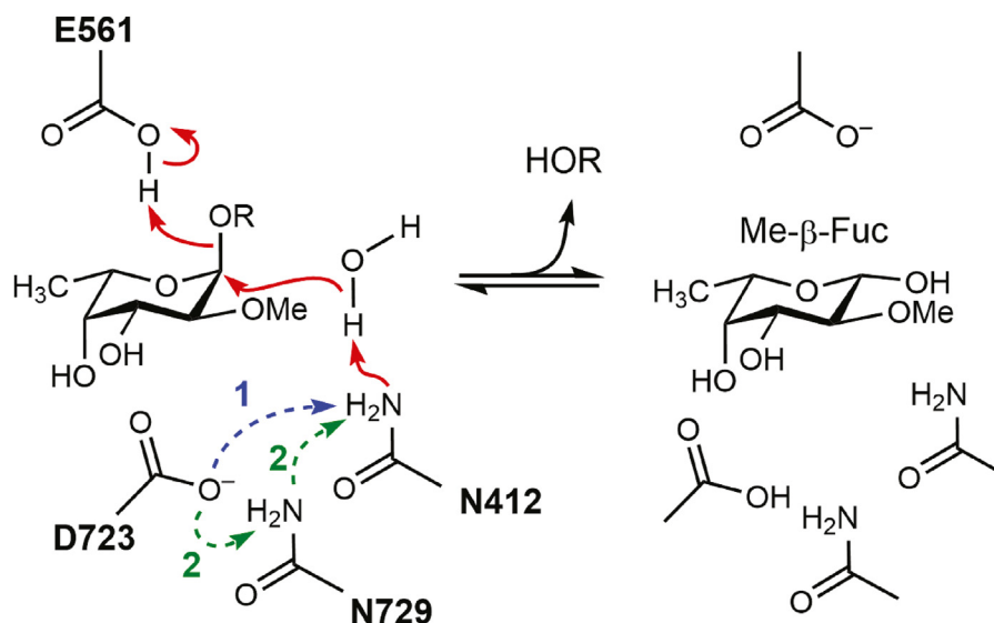
Figure 9. Two proton-transfer pathways that activate Asn412 for nucleophilic water attack in the GH139 inverting mechanism. Schematic of the proposed catalytic cycle for BT0984 GH139 , illustrating two alternative routes by which Asn412 is converted into an effective catalytic base (1). Direct pathway. Asp723 abstracts a proton from the side-chain amide of Asn412. The deprotonated Asn412 then removes a proton from the catalytic water, facilitating nucleophilic attack on the anomeric C1 of \alpha -L-fucose (2). Relay pathway. Asp723 deprotonates Asn729; Asn729 subsequently deprotonates Asn412, which in turn activates the catalytic water. This three-step proton relay mirrors the mechanism proposed for inverting GH45 cellulases (26). In both cases reaction results in inversion of configuration and Glu561 acts as the catalytic acid that protonates the leaving group.
