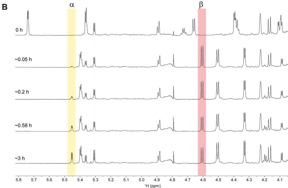
Figure 2. BT0984 GH139 cleaves 2O-methyl- \alpha -fucoside linkages with inversion of stereochemistry. A, the two most common catalytic mechanisms employed by glycoside hydrolases. B, NMR time course of BT0984 GH139 cleavage of \Delta bt0984 oligo in D 2 O. Enzyme concentration and substrate amounts used were 50 \mu M and 0.5 mg in 10 mM HEPES buffer pH 7.0 with 150 mM NaCl.
