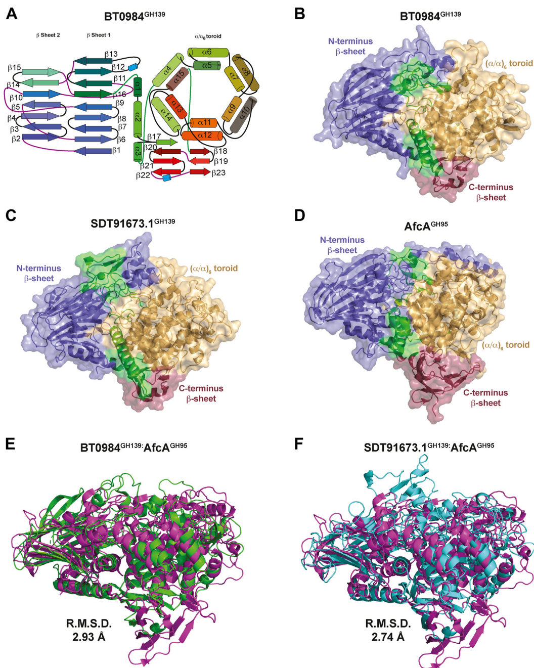
Figure 3. GH139 enzymes share a toroidal (\alpha/\alpha)_6 structure with Afca GH95 . A , cartoon schematic showing the general 3-D structure of GH139 enzymes. B , C , D , transparent surface views of the three enzymes with ribbon diagram of protein structures with the N-terminal domain coloured slate blue, the (\alpha/\alpha)_6 toroid light orange, and the C-terminal domain raspberry red, with interdomain linkers shown in green: ( B ) BT0984 GH139 , ( C ) SDT91673.1 GH139 , and ( D ) Afca GH95 . E , structural overlay of BT0984 GH139 (green) and Afca GH95 (magenta). F , structural overlay of SDT91673.1 GH139 (cyan) and Afca GH95 (magenta).
