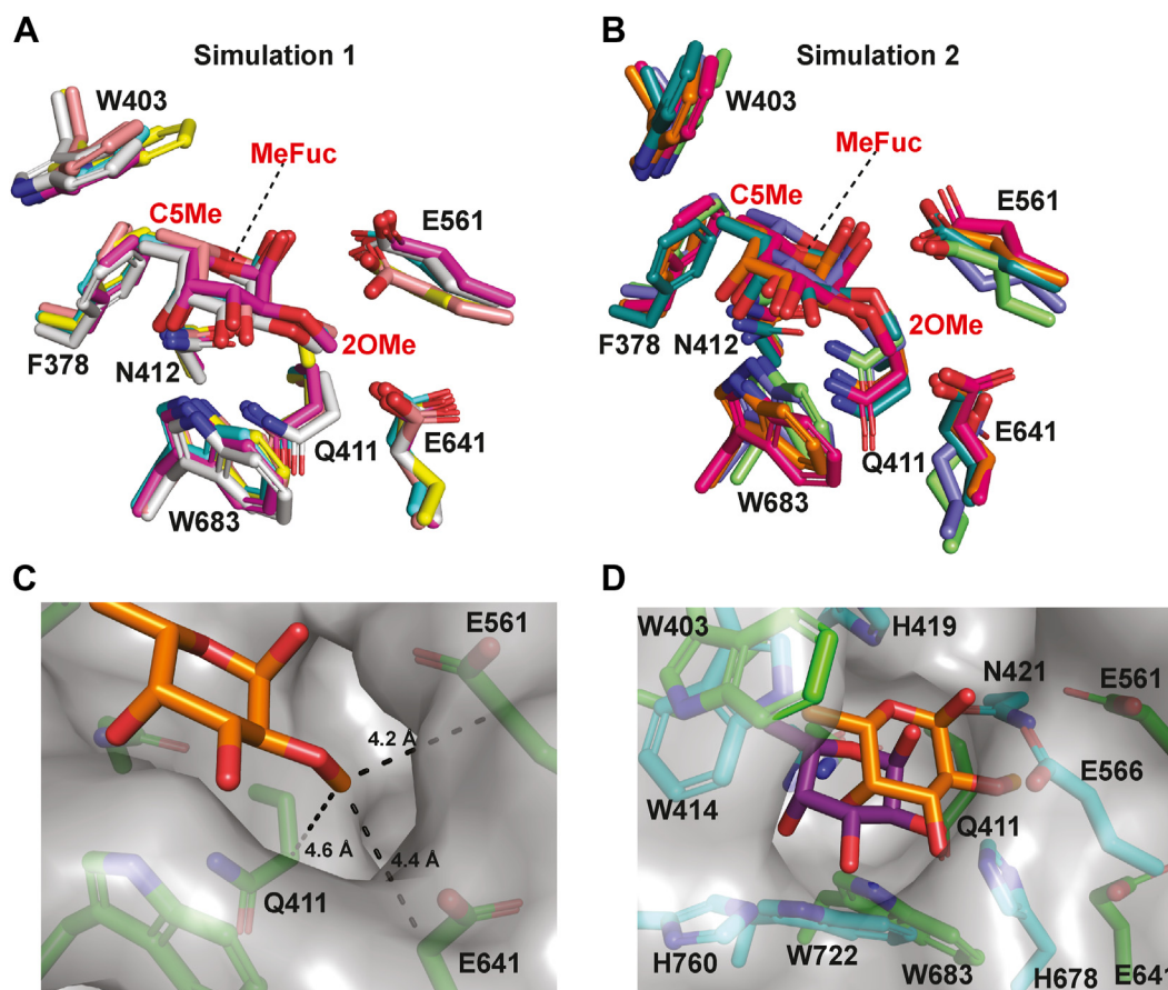
Figure 8. Molecular dynamics simulations reveal the interaction of O2-methyl- \alpha -L-fucose with BT0984 GH139 . A, stick representation of the top five binding poses from molecular dynamics simulation one of BT0984 GH139 in complex with O2-methyl- \alpha -L-fucose. B, stick representation of the top five binding poses from simulation 2. C, surface and stick representation of BT0984 GH139 with O2-methyl- \alpha -L-fucose (pose one from simulation one shown) highlighting the proposed O2-methyl binding pocket. D, overlay of pose 1 (simulation 1), in green with an orange MeFuc, with family GH95 enzyme AfcA (PDB: 2EAC), in cyan, including \alpha -L-fucose (from PDB: 2EAE), in purple, shown as a surface and stick model to illustrate differences in sugar binding poses.
