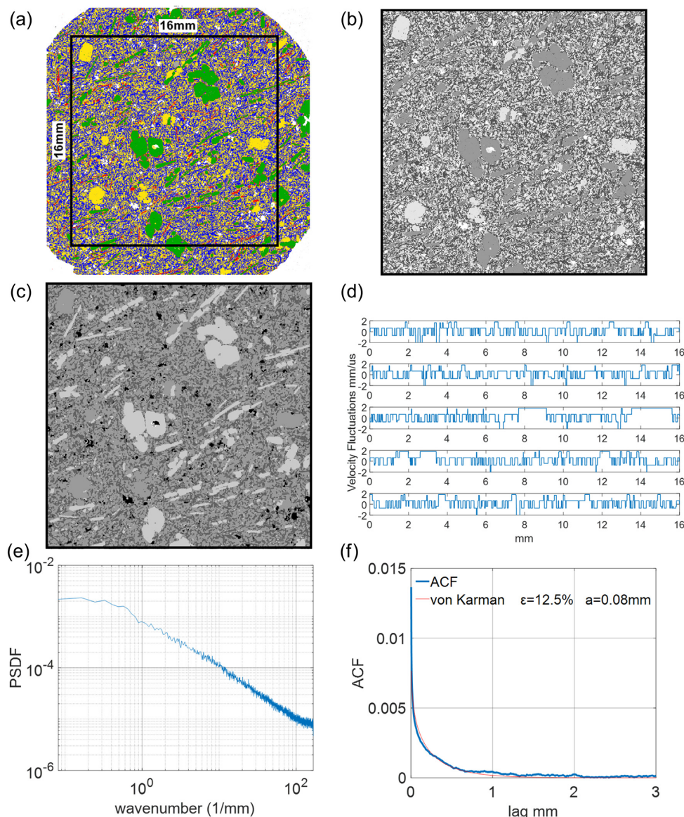
Figure 5. Statistical description of the medium for sample 2H. (a) mineral map; (b) greyscale intensity image of the 256 mm 2 section indicated by the black square in panel a; (c) map of the velocity fluctuations (after filtering), pores in black; (d) example of 5 vertical profiles along with panel c; (e) averaged PSDF and (f) ACF fitted by a von-Karman function, a and \epsilon values are indicated.
