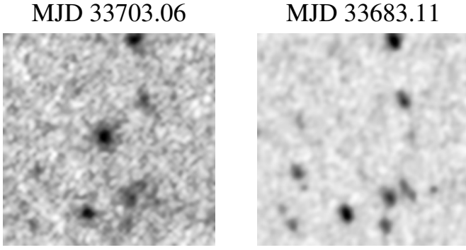
Fig. 2. Harvard photographic plates retrieved via DASCH depicting a historical GOTO0650 superoutburst on MJD 33 703.06 (1951.15) after correcting the alignment for additional distortion. We also show an image taken on MJD 33 683.11 (1951.037).
