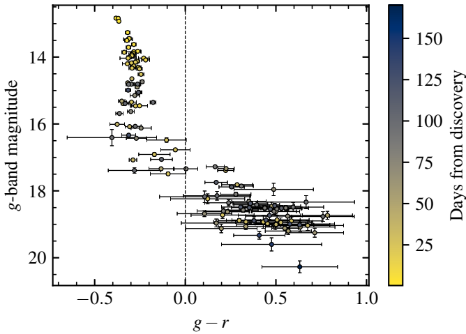
Fig. 5. g - r colour of GOTO0650 as a function of apparent magnitude. The colour scale shows the phase relative to discovery. A clear change in the source colour with magnitude is visible and shows a strong reddening on the way to the low state.
