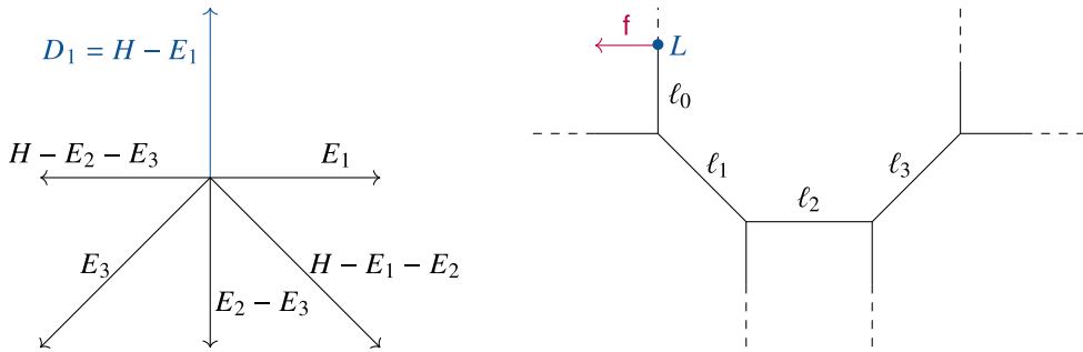
Figure 4. The fan of dP'_3 on the left and the toric diagram of (X, L, f) on the right [11, Figure 6.5].
