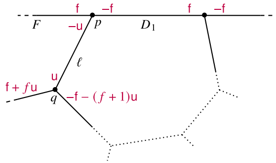
Figure 2. The image of the toric skeleton of Y under the moment map.
