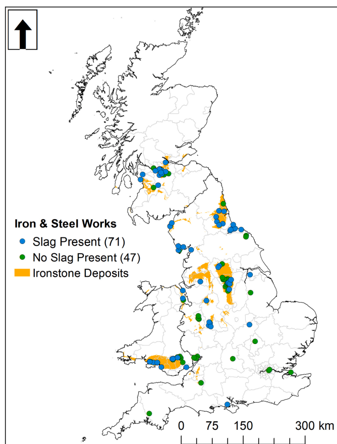
Fig. 1. Locations of historic and current iron and steel works and indication of slag presence presented alongside the location of ironstone bedrock deposits (geological data provided by the British Geological Survey).
