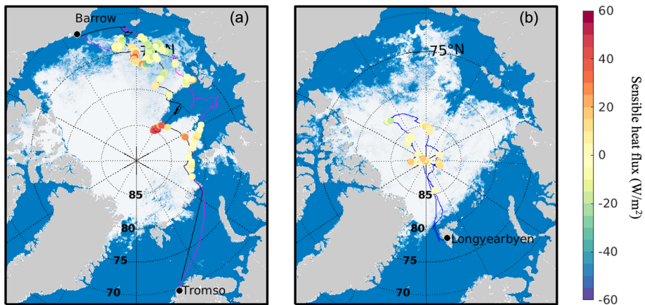
Fig. 1 Maps of the cruise tracks for a ACSE and b AO16. The ice fraction is shown on (a) 07/08/2014 and (b) 07-08-2016. The 30-min mean estimates of turbulent heat flux (positive values indicate an upwards flux) are shown for all points passing the quality control criteria
