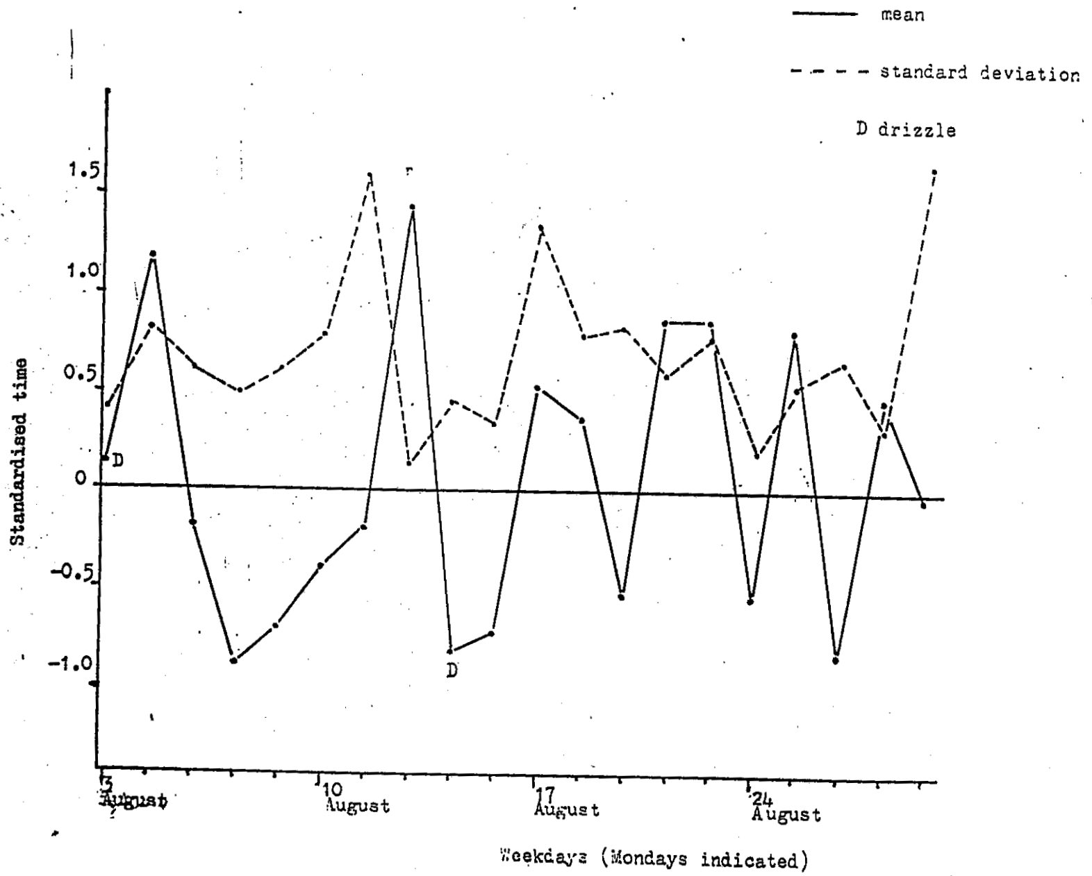
Figure 5(b): Daily variation in mean and standard deviation of standardised travel time (summer)
