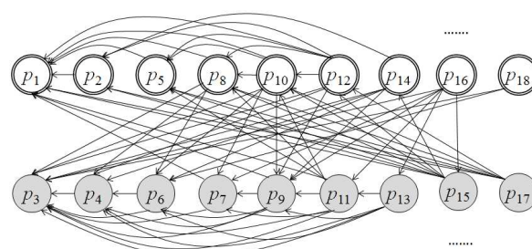
Figure 1. The citation graph of the reachability indexing domain (c.f. the RE data set in Table 1).
