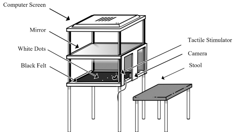
Fig 1. Schematic of augmented reality system with tactile stimulator.
