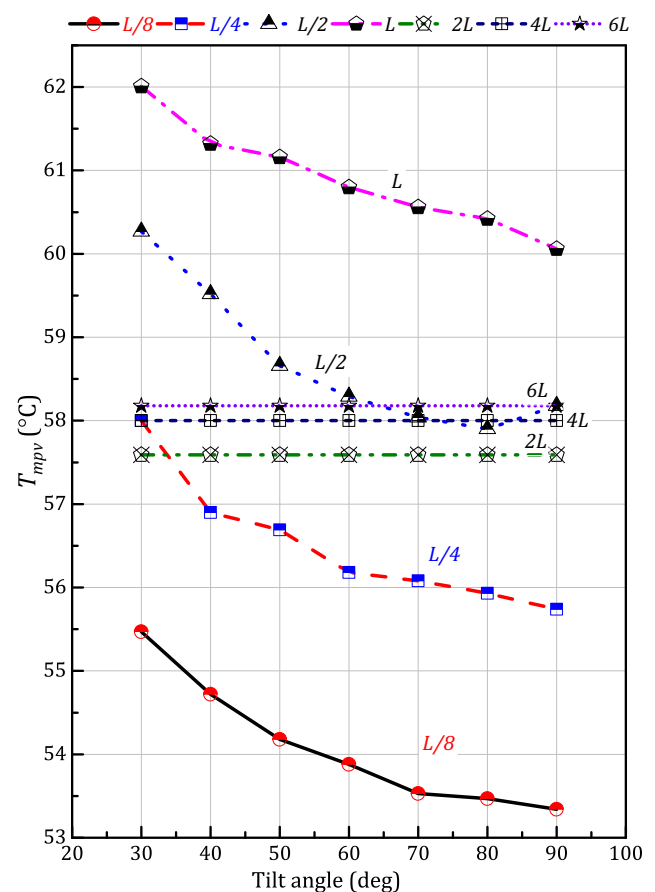
Fig. 7 Tilt angle (in the range 30^\circ - 90^\circ ) versus average PV module temperature with different lengths, predicted using the CFD model for a typical 31st January at 13:00 in Fallujah city.
