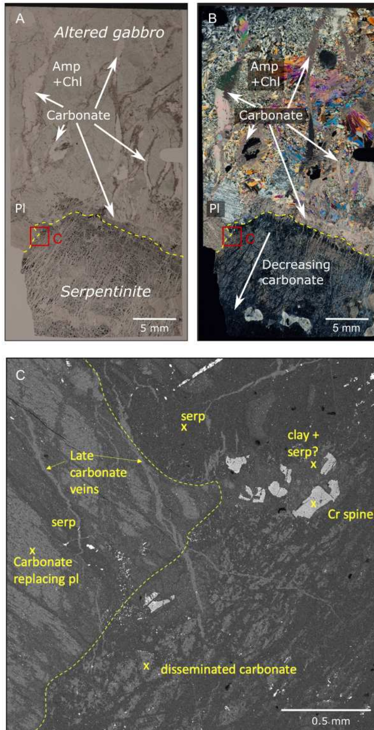
Fig. S16: Extensive carbonate veining and alteration in serpentized peridotite and altered gabbro. Interval 399-U1601C-177R-1, 35-38 cm. (A) Whole thin section image (plane-polarized light) showing carbonate veins cutting gabbro completely altered to amphibole (Amp), chlorite (Chl), clay minerals, and locally secondary plagioclase, in contact with highly serpentized peridotite. The contact is highlighted by the yellow dashed line. (B) Cross-polarized light image
