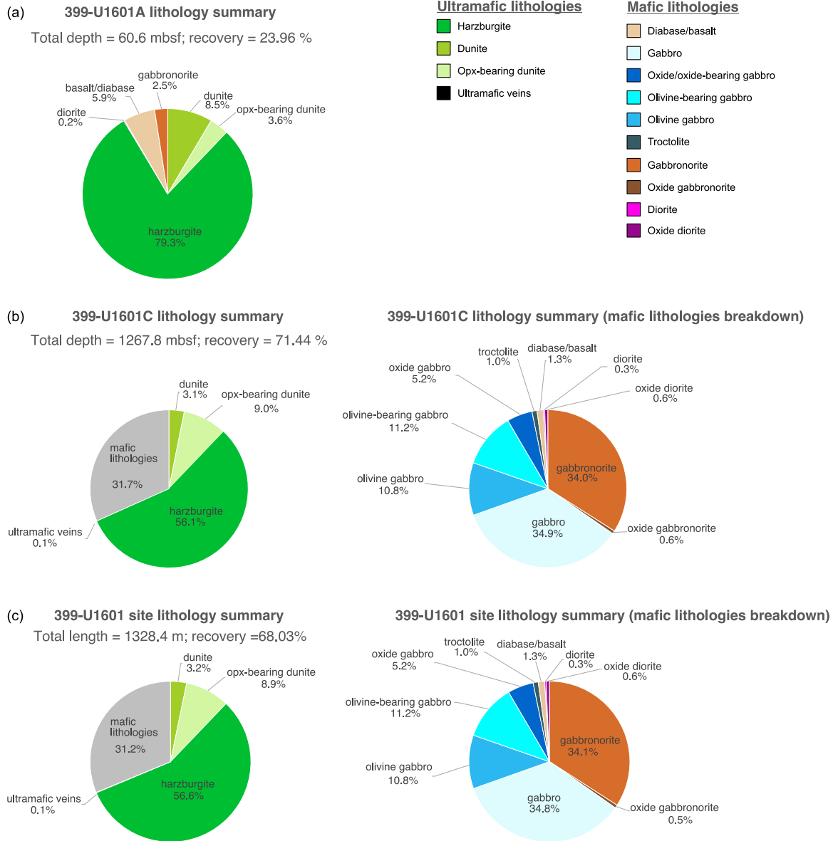
Fig. S4: lithological percentages of rocks recovered from Hole U1601A (A), Hole U1601C (B) and Site U1601 (C).
