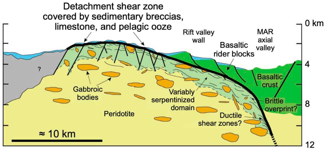
Fig. S2: Cross section of the South wall of Atlantis Massif. The South wall is dominated by variably altered peridotites with gabbroic lenses. Estimated 100 m thick detachment fault zone containing talc-tremolite-chlorite metasomatic schists is at the summit (16). In Expedition 399, the fault zone was found to be <30 m thick. MAR = Mid-Atlantic Ridge. Modified from (66).
