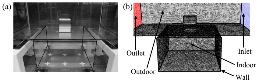
Fig. 2. (a) Closed-loop wind tunnel test set-up; (b) view of the computational mesh of the wind tower and test room model.
