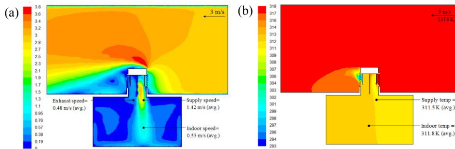
Fig. 4. (a) Velocity contour of a cross-sectional plane inside the test room; (b) temperature distribution inside the test room model
