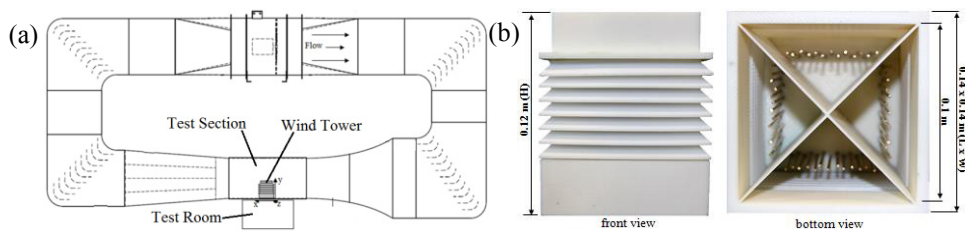
Fig. 3. (a) Closed-loop wind tunnel; (b) 3D printed model of a wind tower with cylindrical HTD (configuration 2).
