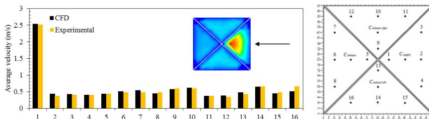
Fig. 6. Comparison between the experimental and CFD results of the airflow velocity measurement
