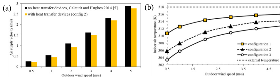
Fig. 5. (a) Effect of the integration of HTD on the air supply velocity (b) Thermal performance of different HTD configurations
