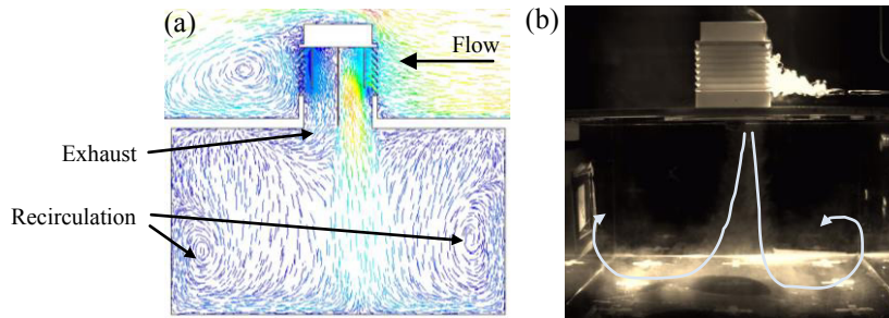
Fig. 7. (a) CFD flow visualisation; (b) Smoke testing in the wind tunnel
