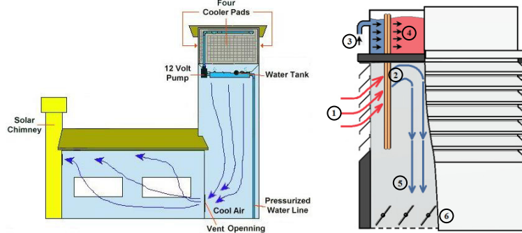
Fig. 1. (a) wind tower with evaporative cooling; (b) wind tower integrated with heat transfer devices (HTD)
