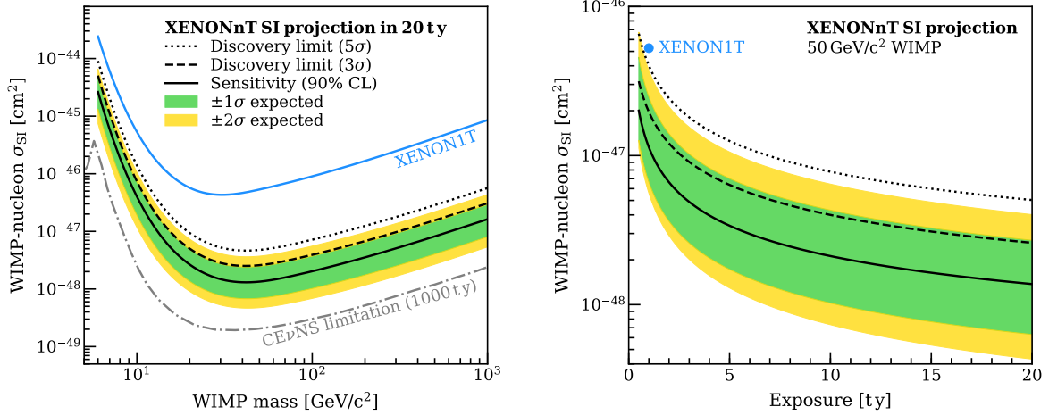
Figure 6: Projections of the XENONnT sensitivity and discovery power in the search for spin-independent WIMP-nucleon couplings. (Left) Median 90% CL exclusion limit (black solid line) for a 20 ty exposure, with the 1\sigma (green) and 2\sigma (yellow) bands. The current strongest exclusion limit, obtained with XENON1T [3], is shown in blue. The gray dashed-dotted line represents the discovery limit of an idealized LXe-based experiment with CE \nu NS as unique background source and a 1000 ty exposure [70]. The improvement of the discovery potential with increasing exposure below that line would be significantly slowed down by the atmospheric neutrino background. (Right) Sensitivity as a function of exposure, for the search of a 50 GeV/c 2 WIMP in the assumed 4 t fiducial mass. The dashed (dotted) black lines in both panels indicate the smallest cross-sections at which the experiment would have a 50% chance of observing an excess with significance greater than 3\sigma ( 5\sigma ). A two-sided profile construction is used to compute the confidence intervals.
