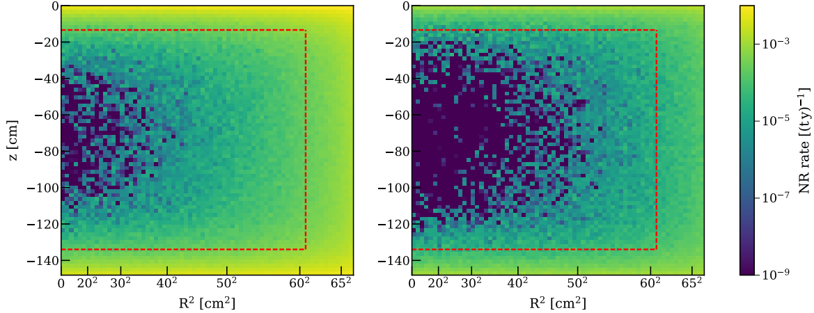
Figure 4: Spatial distribution of the radiogenic neutron background events inside the detector active region, in the (4,50) keV energy window, before (left) and after the NV cut is applied (right). The dashed red line corresponds to the 4 t cylindrical fiducial volume. In this region, the total NR contribution from neutrons corresponds to 0.321 \text{ (ty)}^{-1} without the suppression provided by the NV and 0.041 \text{ (ty)}^{-1} after applying the NV cut.
