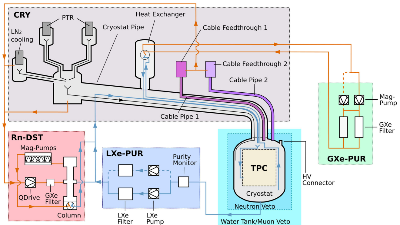
Fig. 2 Schematic drawing of the xenon handling system and the TPC of XENONnT. The circulation of xenon through the purification systems is indicated with orange (GXe) and blue (LXe) flow lines
