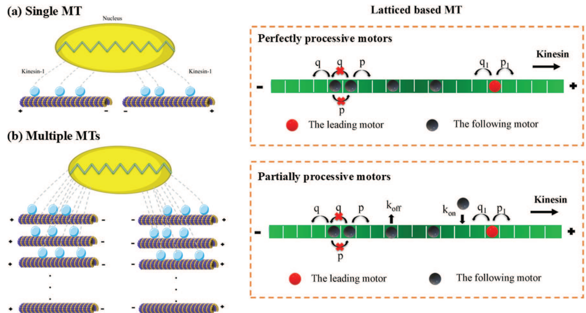
Fig 2. Schematic of tug-of-war between two opposite teams of the same type of molecular motors (kinesin-1, in blue) along (a) one and (b) multiple microtubules. The microtubules on the left are polarised in the opposite direction to those on the right. In the simulation, the microtubules are modelled as a one dimensional lattice on which kinesin-1s are either perfectly processive (never unbind off the microtubules) or partially processive motors (can unbind off the microtubules after one or multiple steps). Kinesin-1 motors on microtubules are connected to the cargo and attempt steps preferentially towards the microtubule plus-end, so the forward stepping rate, p_1 and p , is much larger than backward stepping rate, q_1 and q , for the leading motor and the following motors, respectively. The motors are not allowed to move to an occupied site thus obeying a simple exclusion process. For partially processive motors, they can bind on and unbind off the microtubules with a rate of k_{on} and k_{off} , respectively. The cargo (large yellow ellipse) is allowed to deform elastically using a model of a simple elastic spring with spring constant, k = 0.52 \text{ nN}/\mu\text{m} chosen for a cell nucleus from measurements by Stephens et al [25]. This figure was created using icons from the Reactome Icon Library ( https://reactome.org/icon-lib ), available under a Creative Commons Attribution 4.0 International (CC BY 4.0) license.
