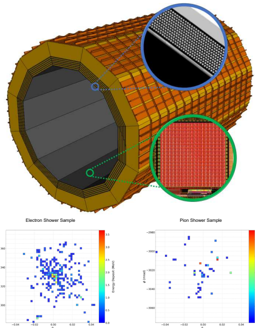
Fig. 7 (top) ECal hybrid concept: the barrel hybrid electromagnetic calorimeter concept for EIC. More details can be found in [54]; (bottom) Projection of Showers in the ECal: Shower projections of electrons (left) and pions (right) as a function of \psi and \eta . Energy deposition in the pixelated array is represented via color, commonly occupying the channel axis in vision-based neural networks.
