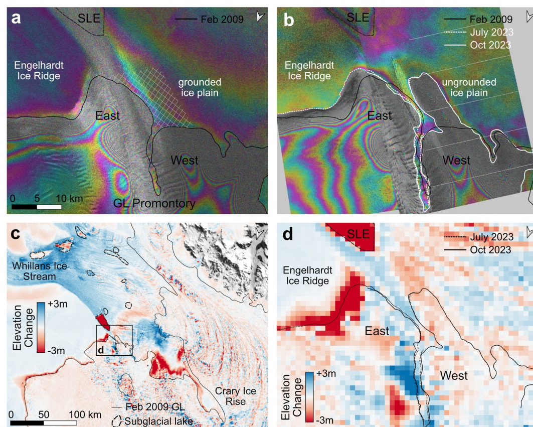
Figure 6. GL migration and surface elevation change downstream of SLE, 2009–24. (a) February 2009 RADARSAT-2 DInSAR and derived GL (black line) showing the east and west embayment and central grounded promontory. White hashed area shows the approx. location of the grounded ice plain identified in Brunt et al. (2010). (b) TerraSAR-X DInSAR and derived GLs from July to October 2023 (white dashed and solid lines, respectively; Marsh et al., 2024). (c) ICESat-2 ATL15 gridded surface elevation change across the wider Gould Coast, 2019–24 (Smith et al., 2024). (d) Zoom of (c) over the same region as (a) and (b) showing the 2023 GL positions.
