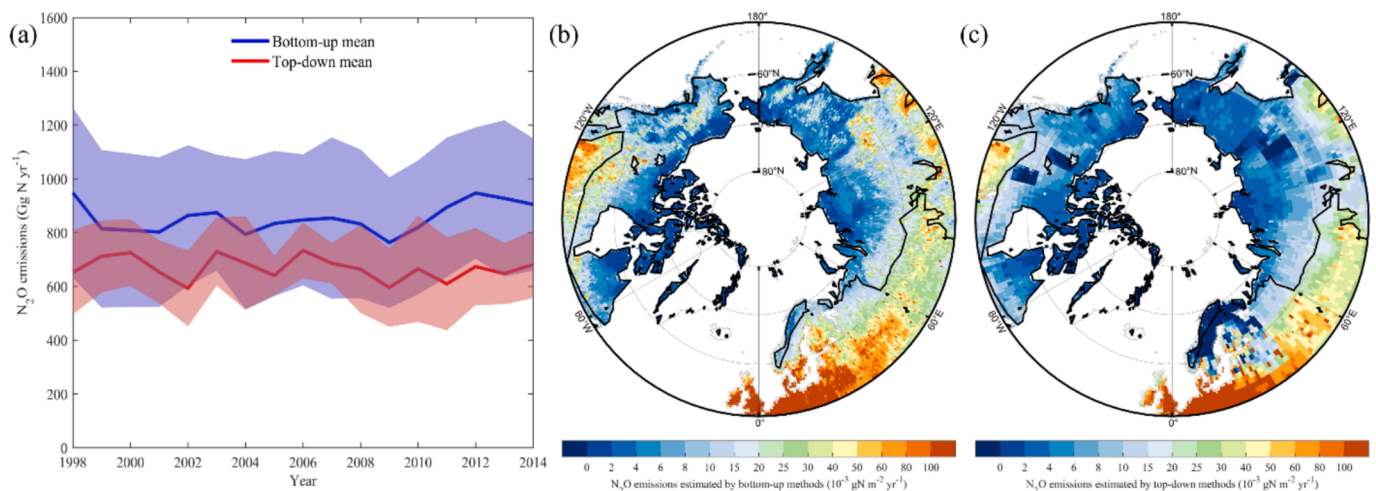
Fig. 4. (a) Comparison between TD and BU estimates of total N 2 O emissions, the lines represent the ensemble means and the shaded areas indicate one standard deviation of model estimates. Spatial pattern of total N 2 O emissions estimated by BU (b) and TD (c) approaches.
