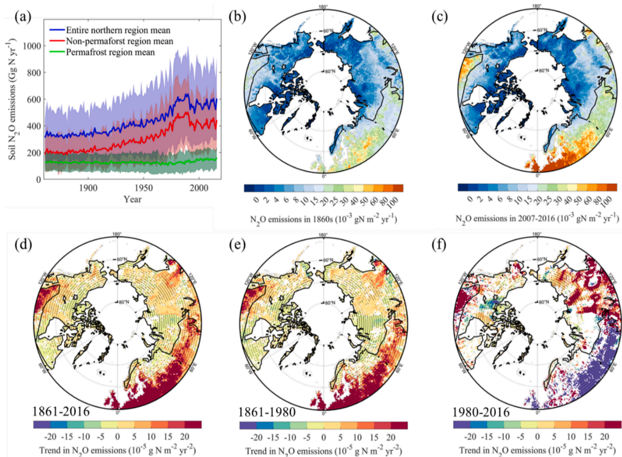
Fig. 1. (a) Changes in soil \text{N}_2\text{O} emissions from the NHL as estimated by NMIP models, the shaded area indicates one standard deviation of all estimates. (b) and (c) show spatial pattern of mean annual soil \text{N}_2\text{O} emissions during the 1860 s and 2007–2016, respectively. Trends in soil \text{N}_2\text{O} emissions during 1861–2016 (d), 1861–1980 (e), and 1980–2016 (f); grids with non-significant trends ( p > 0.05 ) were excluded, and stippling indicates where a majority of models (at least 4 out of 6) agree on the sign of the trend.
