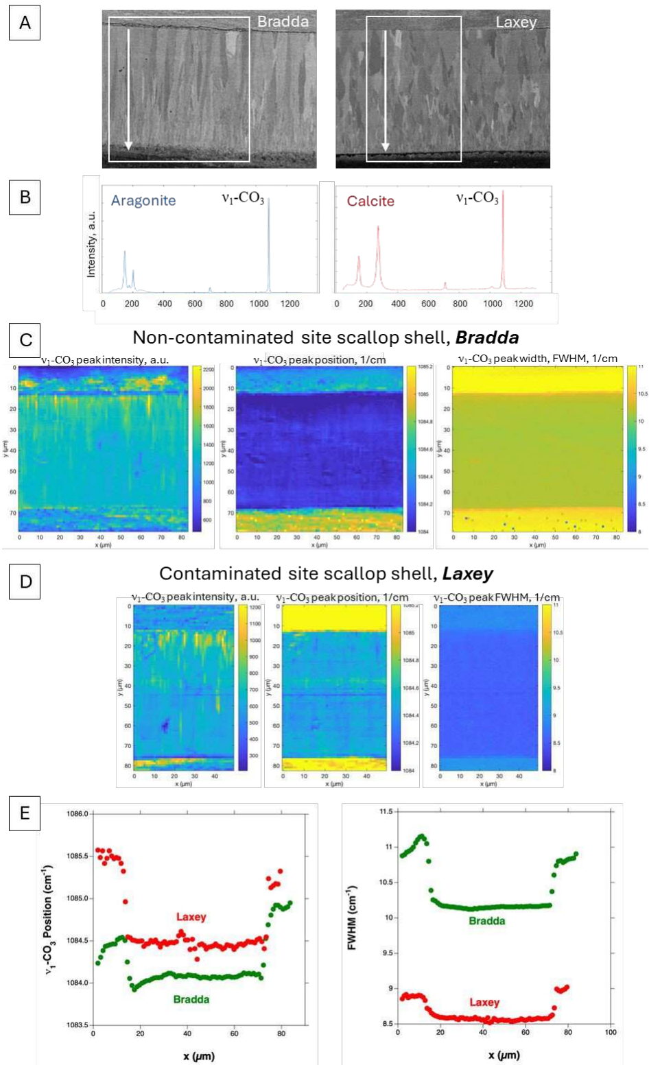
Figure 8: (A) BSE images of a sample from non-contaminated (Bradda) and contaminated (Laxey) sites; (B) Raman spectra taken from the myostracum and foliated regions of the Bradda sample, (C) \nu_1\text{-CO}_3 Raman maps evaluating peak intensity, position and full width at half maximum of the Bradda and (D) and Laxey samples, (E) Comparison of line profiles from top to bottom of the \nu_1\text{-CO}_3 Raman position and full width at half maximum for Bradda and Laxey samples.
