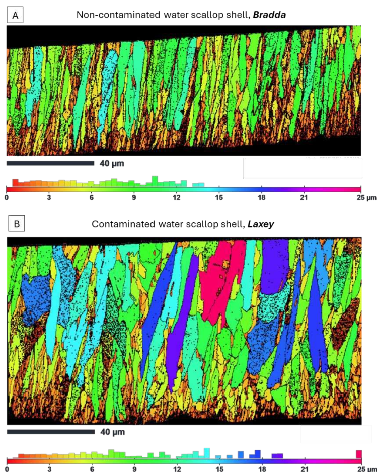
Figure 7 : EBSD grains maps with a color scale according to grain size (longest dimension) in the myostracum.
