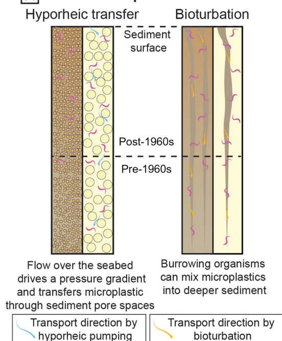
Fig. 9. Synthesis of microfibre transport and burial processes in submarine canyons. (a)–(d) Transport processes. (e) Sub-seafloor processes. (f) Anthropogenic forces. Source: (c) is modified from Chen et al. (2025) .
