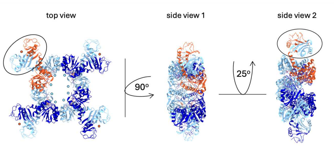
Figure 1 Crystal structure of KtrA.ADP (PDB ID: 4J91; https://doi.org/10.2210/pdb4J91/pdb ). The stoichiometry is a tetramer of dimers. In the top left dimer one monomer is coloured orange, otherwise, the alternating monomers are coloured dark and light blue. The C-terminal region of each dimer protrudes from the core ring and forms the C-lobes (black circle). There are four CDA binding sites, one in each C-lobe (orange circles). There are eight ATP/ADP binding sites, one in the N terminal domain of each monomer (light blue circles). The three views depicted are the views shown in the 2D classes in subsequent figures.
