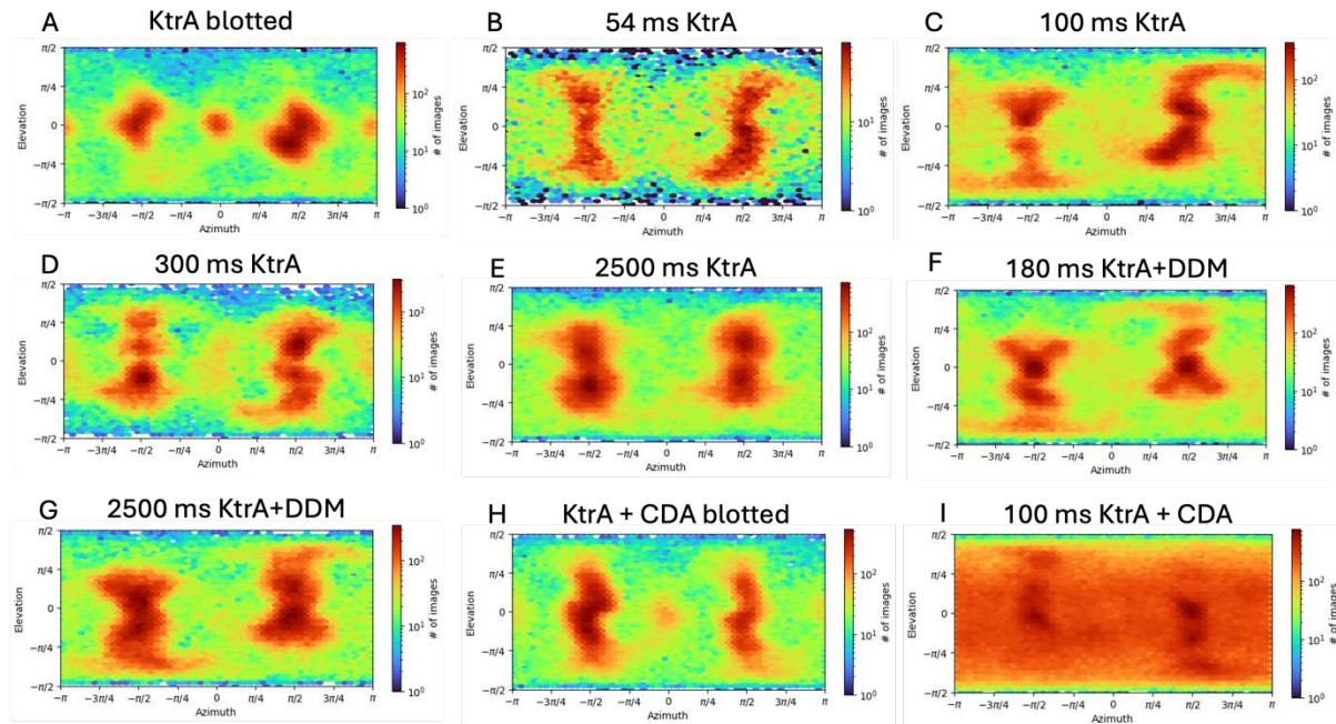
Figure 5 Viewing direction distributions for each sample preparation approach as calculated by cryoSPARC. The combination of a 100 ms plunge time with the addition of CDA leads to the most significant improvement in angular distribution.
