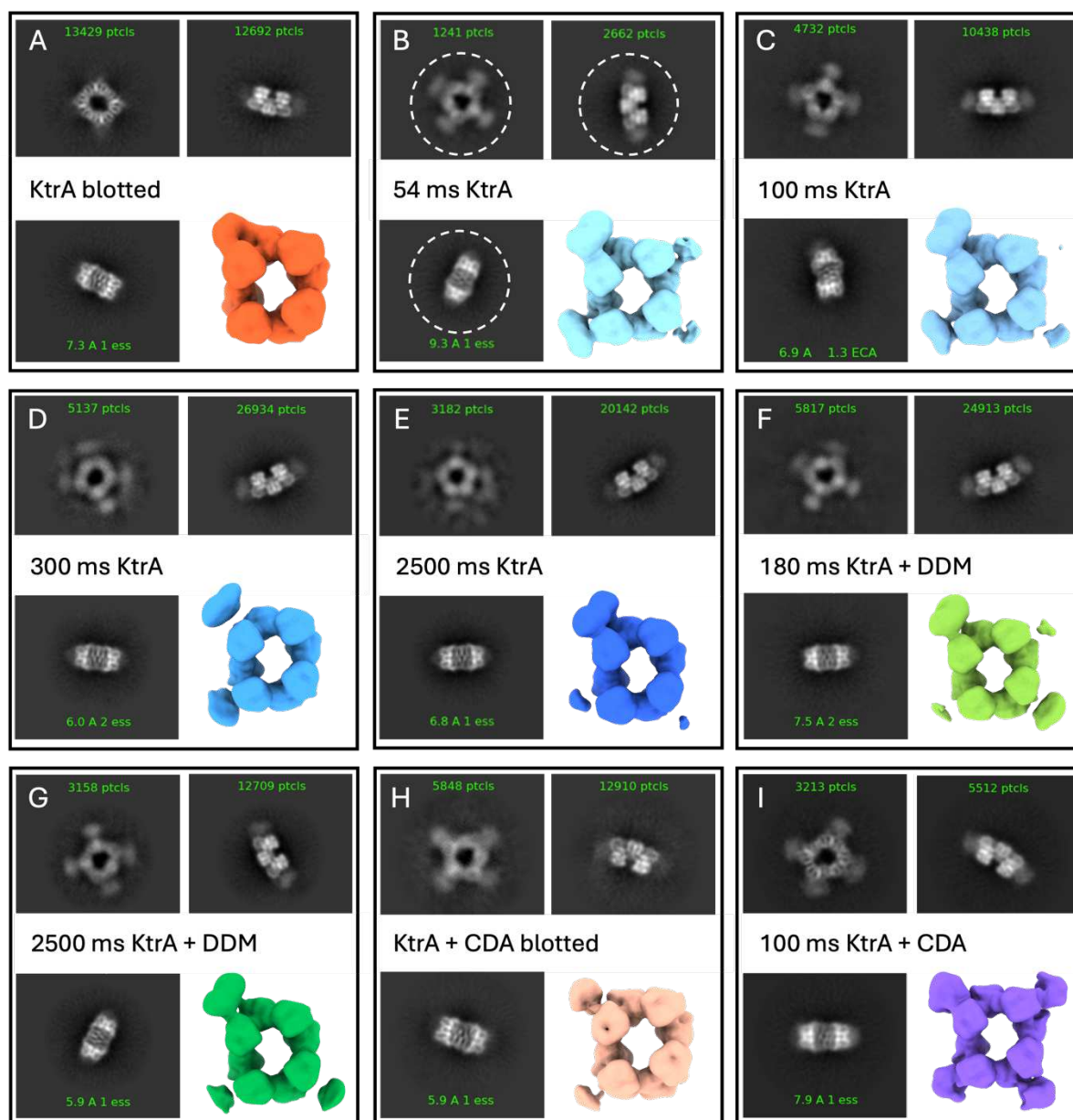
Figure 3 2D classes and 3D density maps for each sample preparation approach. 2D classes of the same three views depicted in Figures 1 and 2 are shown here for each sample preparation condition. Circular mask of at least 200 Å was used for class2D (highlighted with a white dotted circle in B). For each dataset, the top left class is the top view, the bottom left class is side view 1 and the top right class is side view 2. The resultant 3D density map for each condition is also shown. Each map is from a non-uniform refine of 35383 particles. The resulting maps were low pass filtered to 8 Å and visualised in ChimeraX with a normalised threshold.
