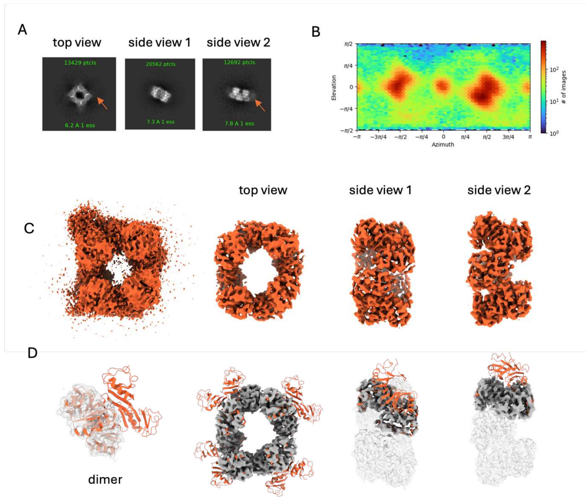
Figure 2 CryoEM results from grid prepared using conventional blotting approach. A) 2D classes of the most populated views, despite secondary structure visible in the core, density for the C-lobes is absent (orange arrows). B) Viewing direction distribution shows there is preferred orientation. C) 3D density map from non-uniform refinement. D) Rigid fit of monomer model from PDB: 4J91 (KtrA.ADP) shows the missing density for the C-lobes.
