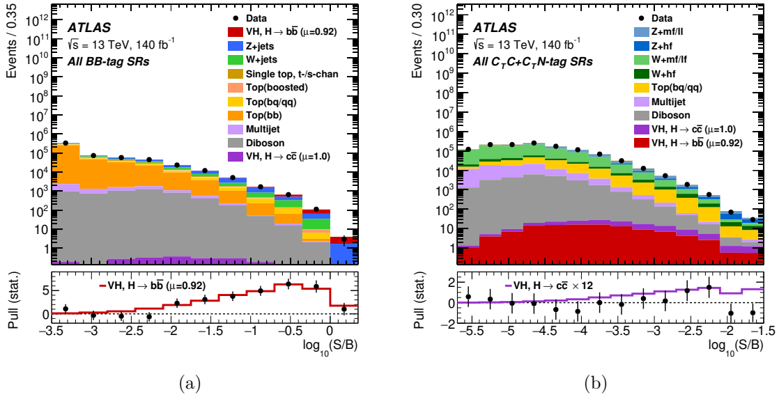
Figure 14. The event yields as a function of \log_{10}(S/B) for data, background and a Higgs boson signal for the nominal VH fit. Final-discriminant bins in the (a) Hb\bar{b} and (b) Hc\bar{c} regions are combined into bins of \log_{10}(S/B) with S being the fitted VH, H \rightarrow b\bar{b} and H \rightarrow c\bar{c} contribution respectively and B the fitted SM background yields. The Higgs boson contributions in the top pad are shown after rescaling the SM cross-section according to the value of the signal strength extracted from data: 0.92 for H \rightarrow b\bar{b} and 1.0 for H \rightarrow c\bar{c} . In the lower panel, the pull of the data relative to the background (the statistical significance of the difference between data and fitted background) is shown with statistical uncertainties only. The full line indicates the pull expected from the sum of fitted signal and background relative to the fitted background; in the H \rightarrow c\bar{c} case, the fitted signal is scaled to the value of the observed upper limit.
