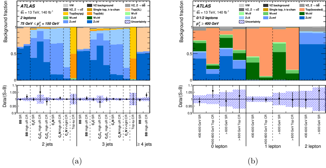
Figure 6. The relative background composition in the signal and control regions with (a) 75 \text{ GeV} < p_T^V < 150 \text{ GeV} in the 2-lepton channel and (b) all regions with p_T^V \geq 400 \text{ GeV} . The ratio of the data to the total signal-plus-background (S+B) prediction is also shown. The background predictions are adjusted with the results of the VH fit to data described in section 9 and the uncertainty band corresponds to the overall uncertainty in the background predictions.
