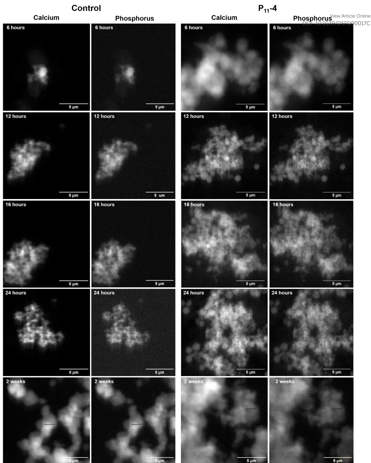
Figure 3: Typical calcium and phosphorus elemental maps at different time points (6 hours, 12 hours, 16 hours, 24 hours and 2 weeks) comparing the control to the mapped SiN windows with deposited P 11-4 , extracted using n-XRF mapping on the I14 beamline. These maps depict the morphology of the formed calcium phosphate structures. The area shown is 15 μm x 15 μm, with a step size of 50 nm.
