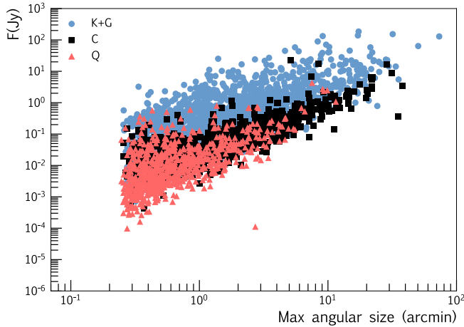
Fig. 9. Flux density of the detected HII regions from the A19 catalogue, as a function of their angular size. Known sources (K) refer to those with measured radio recombination lines (RRLs) or H \alpha emission. Groups (G) are HII region candidates located within the same complex as a known HII region. Candidate sources (C) are those co-spatial with radio continuum emission but lacking RRL or H \alpha detections. Radio-quiet HII regions (Q) are those for which no radio continuum detection was detected in previous surveys.
