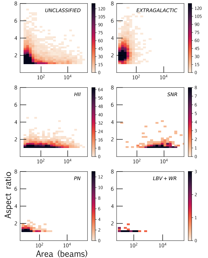
Fig. 8. Bivariate histograms of the source aspect ratio (see text) versus source area. LBVs and WRs are grouped together.
