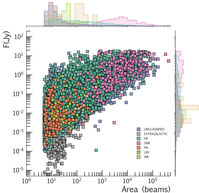
Fig. 4. Scatter plot of flux density as a function of the source area (in beams), coloured by source type. Histograms on the top and right show the marginal source distribution per type relative to each of the variables. Each histogram represents the normalised density function, with normalisation performed independently for each source type to facilitate the visualisation of less represented types.
