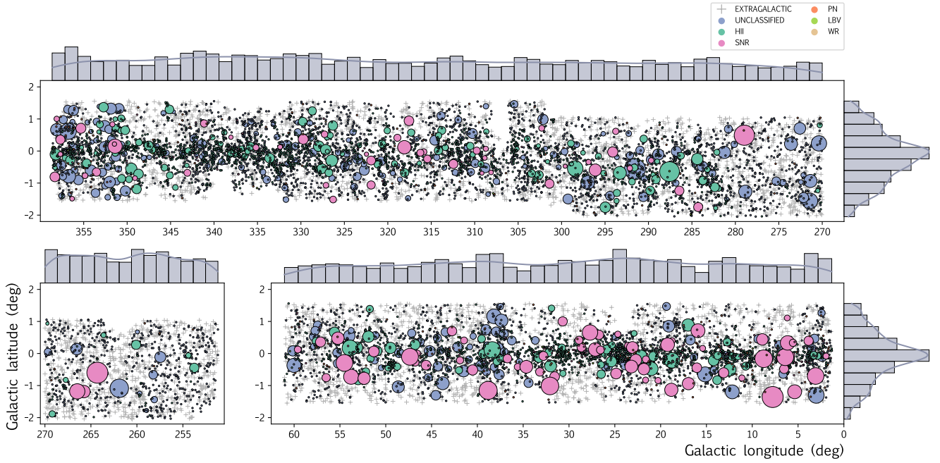
Fig. 3. Sky distribution of the segmented sources in the fourth (top), third (bottom left), and first (bottom right) Galactic quadrants. Extragalactic sources are depicted as grey crosses. Galactic and unclassified sources are represented by circles, coloured by source type (blue=unclassified, bluish green=HII region, magenta=SNR, orange=PN, green=LBV, and brown=WR). Sources with multiple classification tags are not shown. Note the different Galactic longitude coverage in each panel. The source distribution in the fourth quadrant shows a latitude jump around l = 300^\circ due to the SMGPS footprint following the Galactic warp. Sources with an angular radius of less than 10 arcmin are represented with points of fixed size for easier visualisation. Larger sources are represented with larger circles (scaling \propto r^{1.2} ). The histograms to the top and right of each panel represent the marginal distribution of sources in each direction (for the first and third Galactic quadrants, the cumulative latitudinal distribution is shown).
