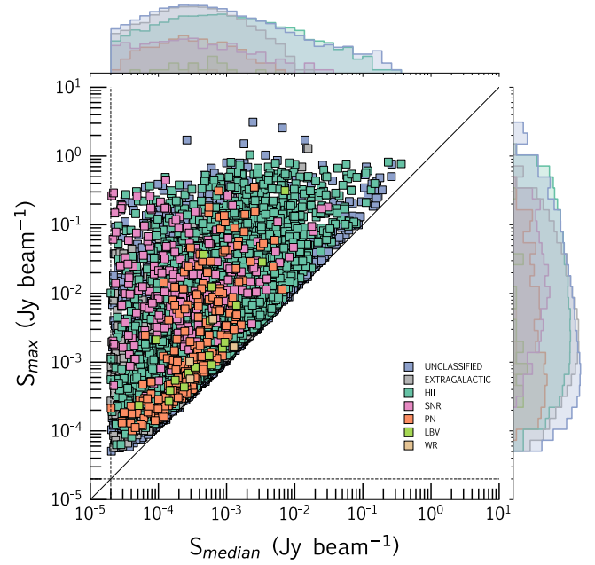
Fig. 6. Scatter plot of the peak and median source brightness, coloured by source type. Histograms on the top and right show the counts per source type relative to each of the variables, in log scale. The solid line represents S_{\max} = S_{\text{median}} , and the dashed lines indicate the upper limit of the nominal off-source rms (10–20 \mu\text{Jy beam}^{-1} ; Goedhart et al. 2024). Sources with median source brightness below this threshold (e.g. due to negative bowls) have been excluded from the plot.
