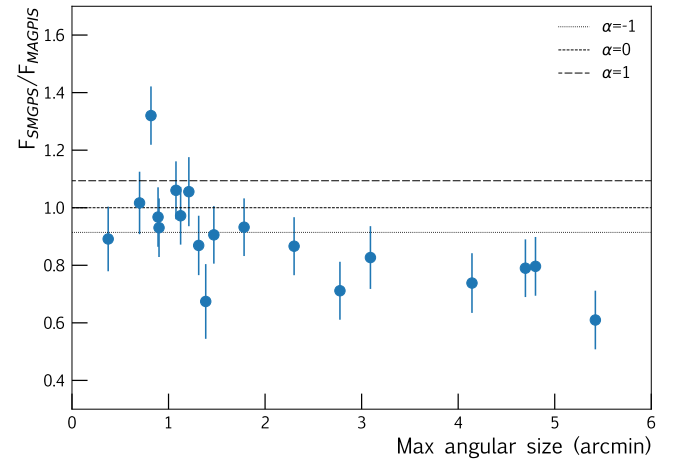
Fig. 7. Comparison of the SMGPS (1.284 GHz) and MAGPIS (1.4 GHz) flux densities for selected sources (blue dots) as a function of the source maximum angular size found in MeerKAT. Dashed lines represent the expected flux ratios for sources with a power-law spectrum of spectral indices \alpha = -1, 0, 1 .
