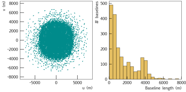
Fig. A.1. Left: Simulated MeerKAT uv coverage for a \sim 1 h pointing at \delta = -30^\circ , split over 10 hours to approximate the real SMGPS coverage. Right: Histogram of baseline lengths ( N=2016 baselines).
