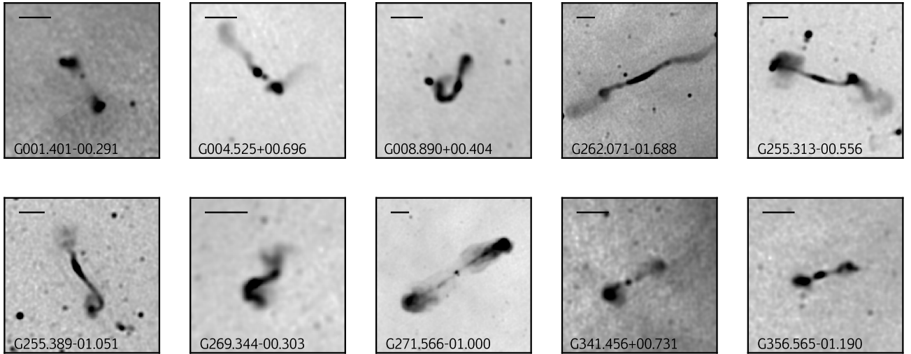
Fig. 11. Examples of SMGPS sources labelled ‘EXTRAGALACTIC’ due to their morphological features. The catalogue source name appears in the bottom-left corner of each panel, and the scale bar in the top-left corner indicates 1 arcmin.
