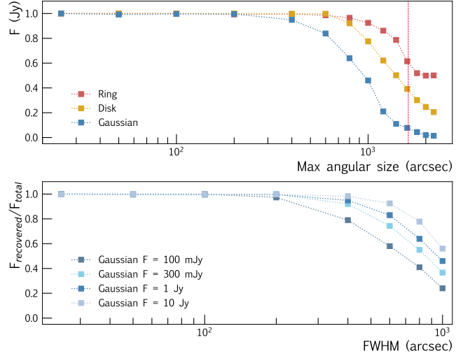
Fig. A.2. Top: Recovered flux density as a function of the maximum angular size for a uniform disk, a ring, and a Gaussian source of F = 1 Jy. The dashed vertical line represents 27 arcmin, the theoretical LAS at the representative frequency of the maps. Maximum angular size refers to the diameter (disk), outer diameter (ring), and full width at half maximum (Gaussian). Bottom: Flux density recovery performance for Gaussian sources of 100 mJy, 300 mJy, 1 Jy, and 10 Jy.
