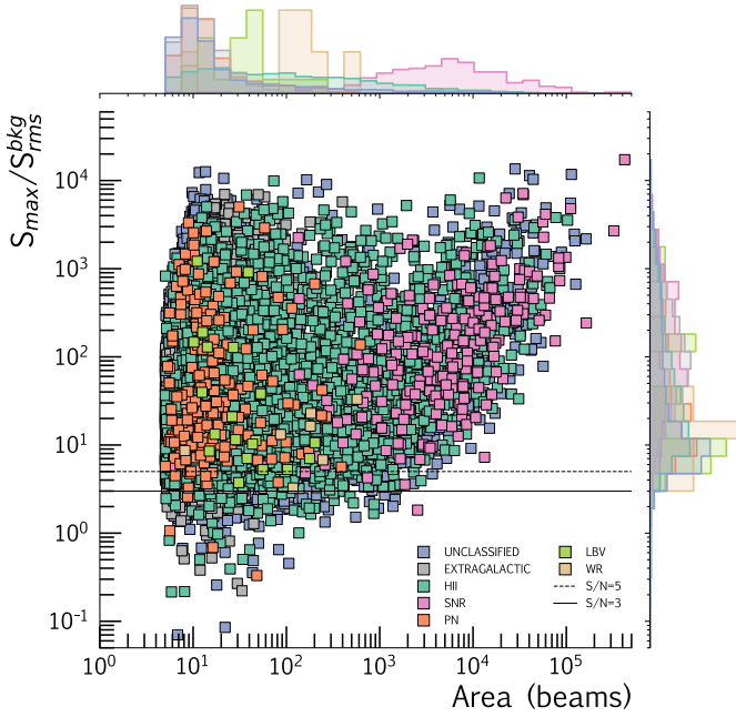
Fig. 5. Scatter plot of the ‘peak’ S/N, i.e. S_{\max}/S_{\text{bkg}}^{\text{rms}} as a function of the source area, coloured by source type. The solid and dashed lines represent the S/N=3 and S/N=5 levels, respectively. Histograms are normalised as in Fig. 4.
