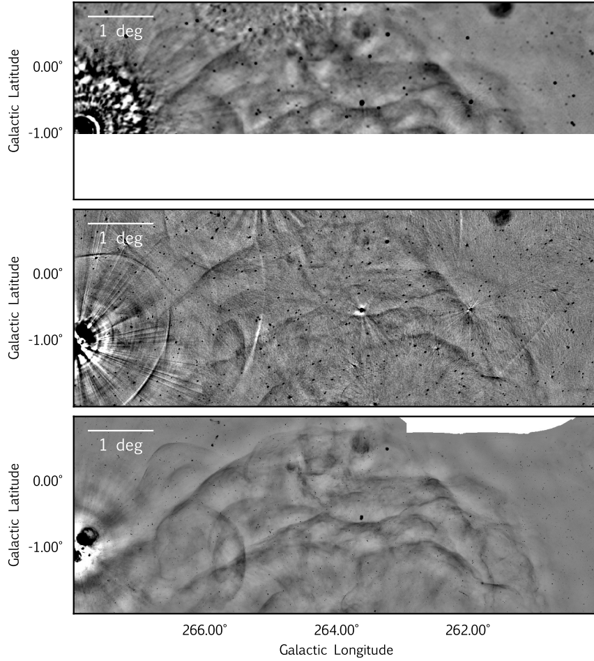
Fig. 10. Vela XYZ SNR, as seen by SGPS (top), MGPS (middle), and SMGPS (bottom).
