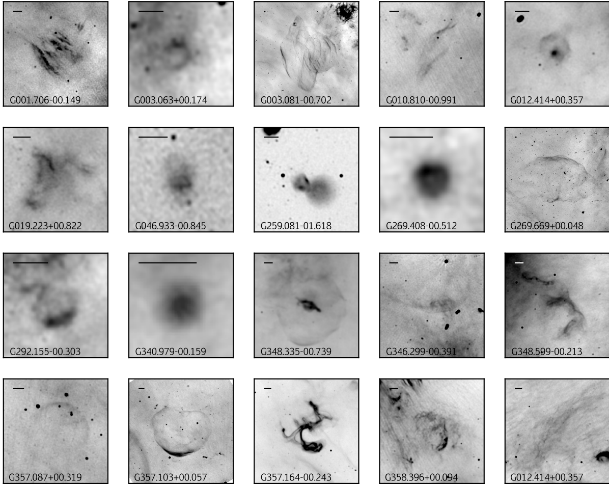
Fig. 12. Examples of SMGPS sources labelled ‘UNCLASSIFIED’. The catalogue source name appears in the bottom-left corner of each panel, and the scale bar in the top-left corner indicates 1 arcmin.
