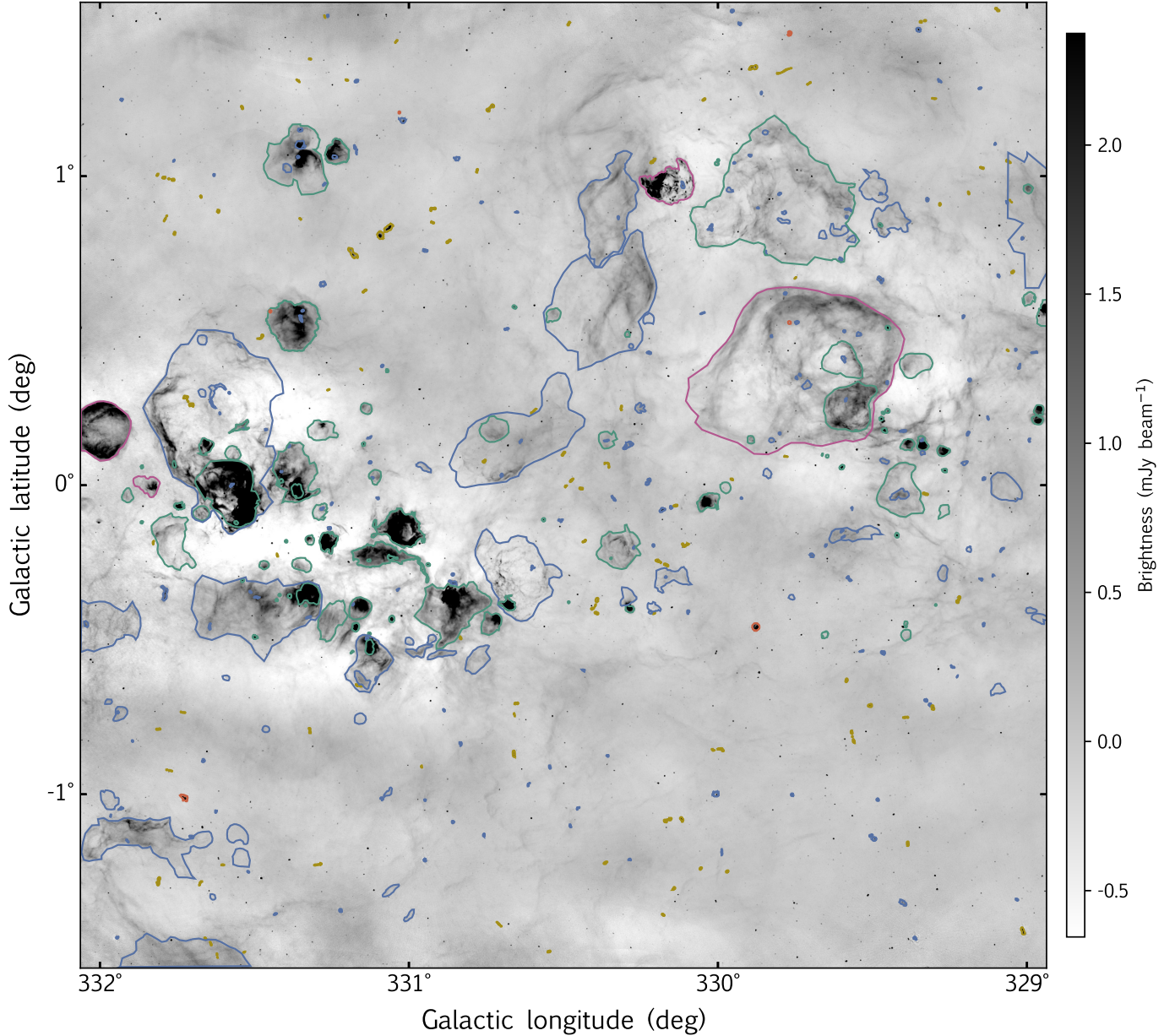
Fig. 1. Example of a fully segmented tile (G330.5+0.0). The sources are coloured according to their assigned tag: magenta=SNR, bluish green=HII region, orange=PN, blue=unclassified, gold=extragalactic. Isolated filamentary structures are excluded from the extended source catalogue.
