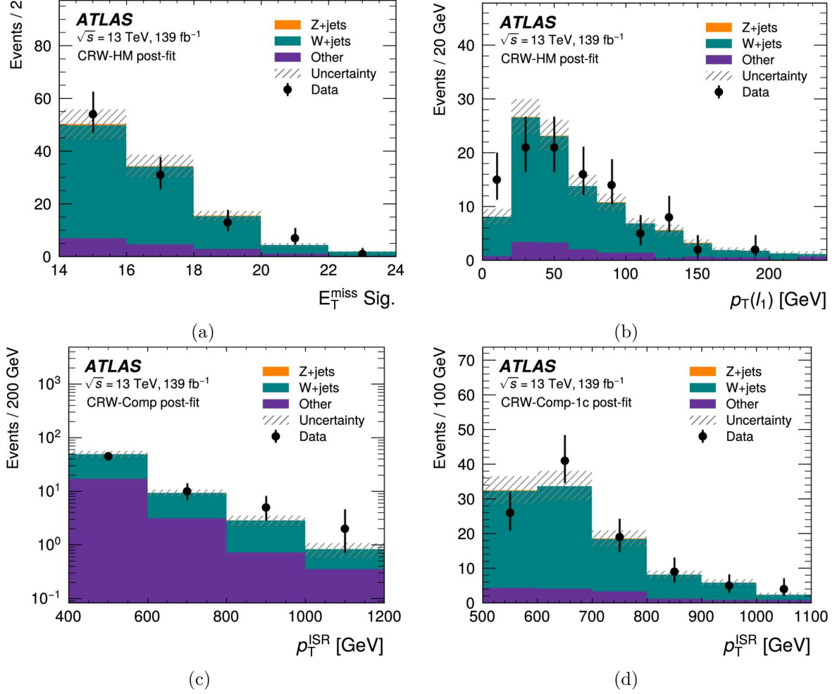
Figure 4. Distributions showing the level of agreement between the data (points) and the SM expectation (stacked histograms, after simultaneously fitting the Z +jets and W +jets backgrounds) in the W +jets control regions for some variables which have different selection criteria in the signal regions: (a) E_T^{\text{miss}} Sig. in CRW-HM, (b) p_T of leading lepton in CRW-HM, (c) p_T^{\text{ISR}} in CRW-Comp, and (d) p_T^{\text{ISR}} in CRW-Comp-1c. The hatched uncertainty band around the total SM expectation includes theory-based and detector-related systematic uncertainties and MC statistical uncertainties. Processes with top quarks and multiple vector bosons are included in “Other”. The Z +jets background contribution is negligible and not visible in the plots. The right-most bin in each histogram does not include the overflow entry but the x -axis range is chosen to include all observed data.
