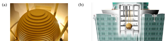
Fig. 1. The tuned-mass-damper (TMD) showing (a) a photograph of the 660-tonne mass from the Taipei 101 tuned-mass-damper, and (b) the mass is suspended on cables, across four storeys at the top of the building acting like a pendulum version of the TMD. A review of TMDs with a list of applications to buildings is reported in Gutierrez and Adeli [1]. Photo credits: Guillaume Paumier
