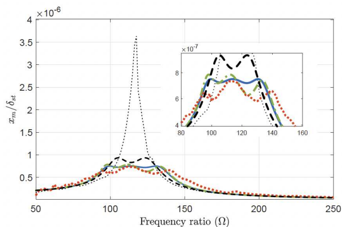
Fig. 7. Experimental results (red dashed line) of the host structure with the prototype inerter device with a mass ratio of 0.045 and a parasitic mass ratio of 0.054 in comparison with the experimental result of the uncontrolled host structure compared to numerical simulations: The uncontrolled structure (thin black dashed line); tuned-mass-damped (thick black dashed line); inerter device with k_{\text{notch}} = 0 (blue line); inerter device with k_{\text{notch}} = 9000 N/m (green dashed line). Full details are given in [32]
