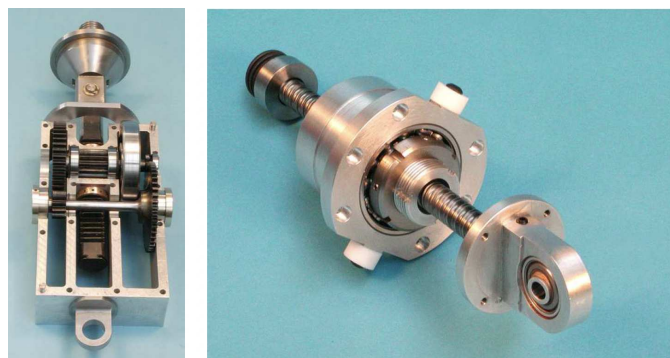
Fig. 2. Mechanical inerter concepts designed by Papageorgiou and Smith [4]. On the left is a rack and pinion inerter, and on the right is a ball-screw inerter. Photo credits: Papageorgiou and Smith [4]
