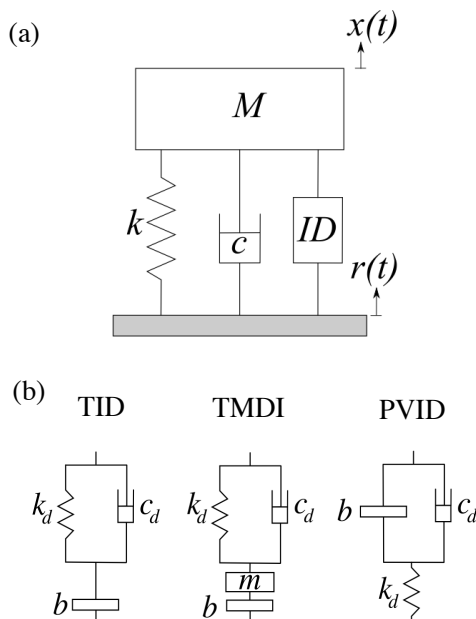
Fig. 3. Tuned inerter device layout variants showing: (a) The host system with mass M , stiffness k , and damping c , and inerter-device denoted ID , the base displacement input is r(t) and the system displacement response is x(t) . (b) Three variants of inerter device; tuned-inerter-damper (TID); tuned-mass-damper-inerter (TMDI); parallel-viscous-inerter-damper (PVID), also sometimes called a tuned-viscous-mass-damper (TVMD). The inerter element has inertance b , the ID has mass m , stiffness k_d and damping c_d
