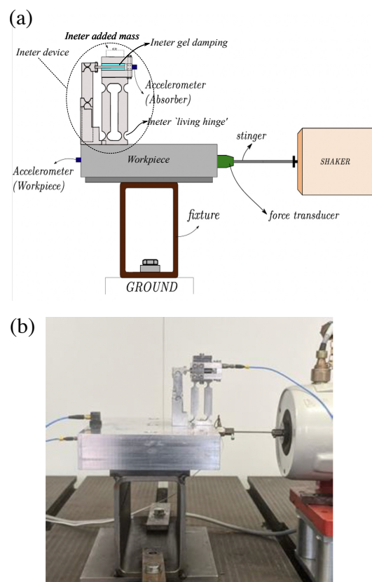
Fig. 6. Experimental setup of the host structure with the prototype inerter device showing: (a) a schematic of the experimental test with the prototype inerter device mounted on the aluminium block which in this setup, and shaker attached (b) an image of the experimental setup. Full details are given in [32]
