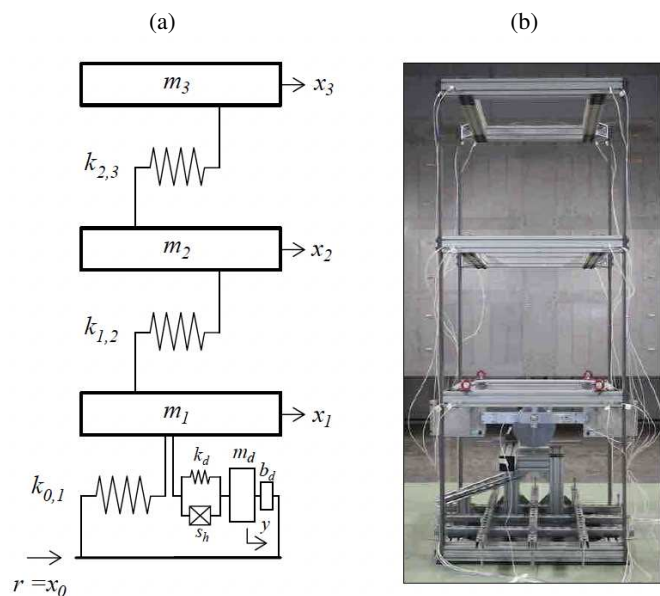
Fig. 4. Three-storey structure inerter experiments showing: (a) lumped-mass model (b) 3-storey experimental test structure with tuned-viscous-mass-hysteretic-damper (TMhDI) fitted between the base and first storey. The masses of each storey are m_1 , m_2 and m_3 , and the stiffness between the storeys are k_{0,1} , k_{1,2} , k_{2,3} . The base structure is assumed to be undamped. The inerter-device parameters are mass m_d , inertance b_d , stiffness k_d and hysteretic damping s_h . The displacement of the inerter-device mass is denoted by y . Full details are given in [31]
