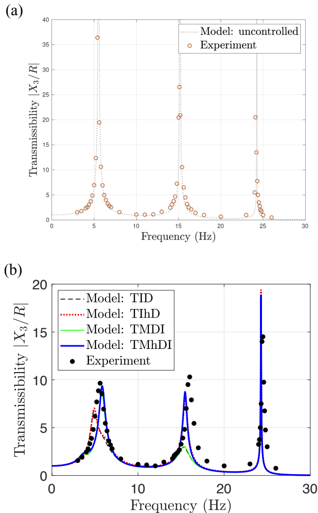
Fig. 5. Results of the three-storey structure with the inerter-based device tuned to suppress the first resonance showing: (a) The uncontrolled structure top storey transmissibility |X_3/R| where X_3 and R are the displacement amplitudes of x_3 and r respectively. (b) The structure top storey transmissibility when equipped with different inerter devices. For full details see [31,35]
