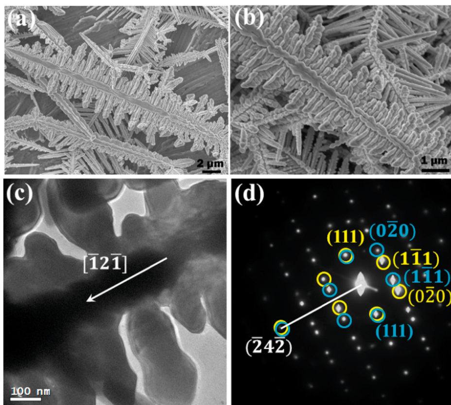
Fig. 8. (a) and (b) SEM images of copper dendrites prepared in a solution with 50 mM of \text{CuSO}_4 and 150 mM of HCl whose secondary branches are perpendicular to the primary trunk. (c) TEM image of such a dendrite. The arrow indicates the growth direction of the trunk. (d) The corresponding SAED pattern. The two sets of diffraction spots circled in yellow and in blue respectively have a mirror symmetry, indicating a twin defect (the white line can be regarded as the location of the twin plane).
