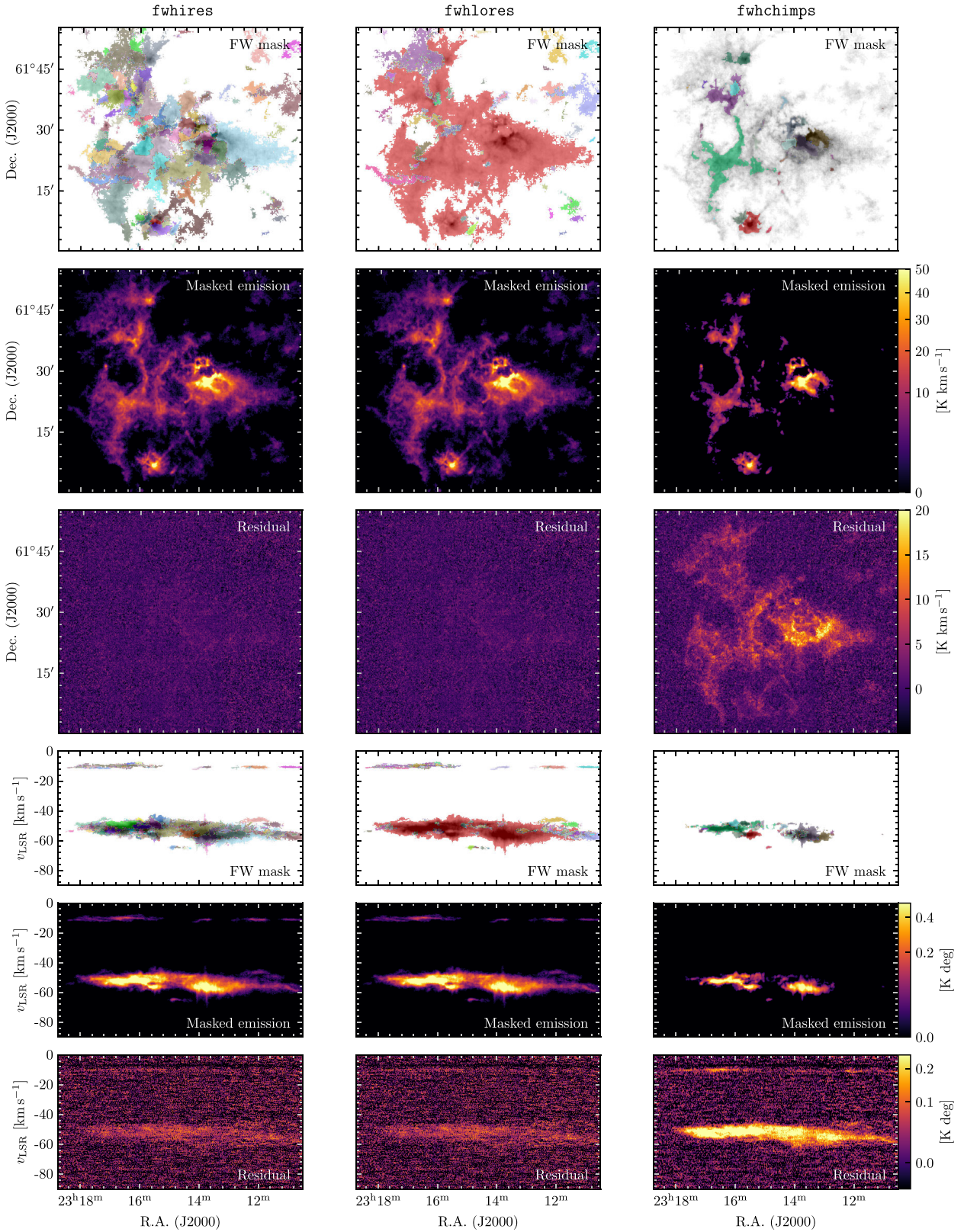
Figure 6. Each column of images shows different aspects of the fwhires , fwlores , and fwhchimps FELLWALKER source-extraction setups. Top row: A greyscale representation of the ^{13}\text{CO} (3–2) velocity-integrated intensity map of NGC 7538 overlaid with 2D representations of the FELLWALKER masks. Second row: Velocity-integrated intensity images from the FELLWALKER-masked cubes. Third row: Residual velocity-integrated intensity map. Fourth row: A greyscale representation of the ^{13}\text{CO} (3–2) declination-integrated position-velocity map overlaid with 2D representations of the FELLWALKER masks. Fifth row: Declination-integrated position-velocity maps of the masked cubes. Bottom row: Residual declination-integrated position-velocity maps of the masked intensity. The images in each row are all on the same intensity scale, indicated by the colour bar on the right-most image.
