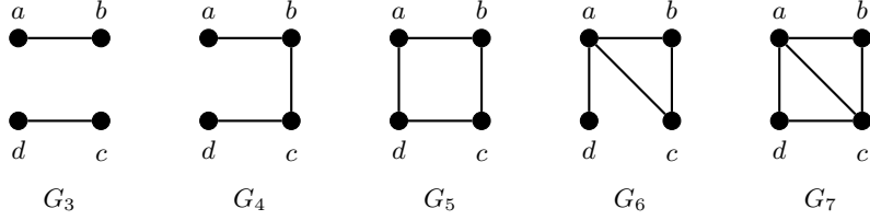
FIGURE 1. The graphs whose edges give the proper, nonempty feasible sets of U_3, U_4, U_5, U_6, and U_7, respectively.
