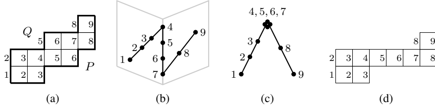
FIGURE 2. Examples of (a) the region of interest, (b) the lattice path matroid it gives, which is the transversal matroid that has the presentation \{\{1, 2, 3\}, \{2, \dots, 6\}, \{5, \dots, 8\}, \{8, 9\}\} , (c) a quotient of that matroid, and (d) a region that yields the quotient.
