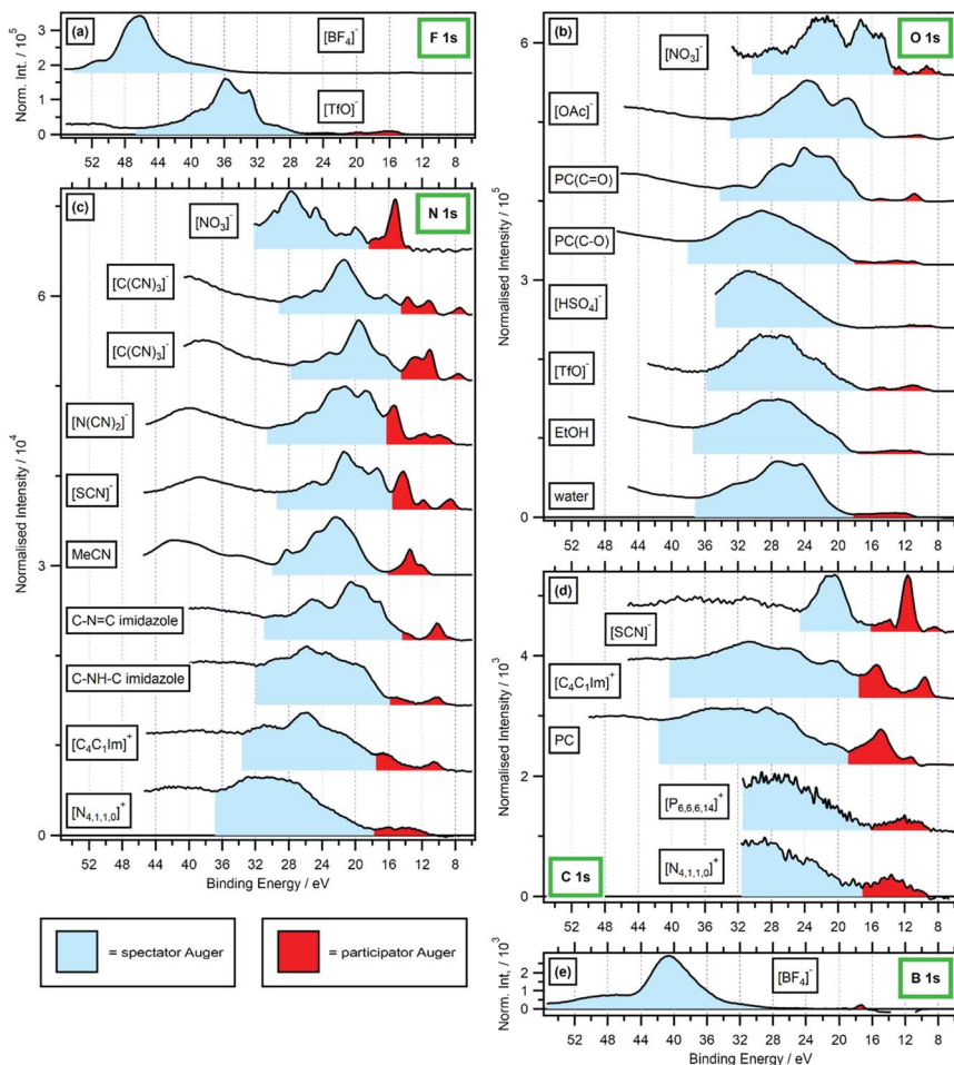
Fig. 4 Valence XPS at different absorption edges. Shaded regions are shown for estimated spectator Auger (SA, in light blue) and participator Auger (PA, in red) transition contributions; backgrounds have not been included, so the SA region in particular will give an overestimate of the true SA area. (a) F 1s valence XPS for 0.5 M [C_4C_1Im][TfO] in water ( h\nu = 690.6 eV) and 0.5 M [C_4C_1Im][BF_4] in water ( h\nu = 696.4 eV). (b) O 1s valence XPS for [P_{6,6,6,14}][NO_3] ( h\nu = 531.9 eV), 1.3 M [C_4C_1Im][OAc] in water ( h\nu = 532.7 eV), propylene carbonate (PC, h\nu = 533.3 eV for C=O absorption and h\nu = 536.2 eV for C–O absorption), [N_{4,1,1,0}][HSO_4] ( h\nu = 536.8 eV), [N_{2,2,1,0}][TfO] ( h\nu = 535.3 eV), ethanol (EtOH, h\nu = 535.4 eV) and water ( h\nu = 535.0 eV). (c) N 1s valence XPS for [P_{6,6,6,14}][NO_3] ( h\nu = 405.2 eV), [C_8C_1Im][C(CN)_3] ( h\nu = 399.0 eV and h\nu = 400.0 eV), 0.5 M [C_4C_1Im][N(CN)_2] in water ( h\nu = 400.1 eV), 0.5 M [C_4C_1Im][SCN] in water ( h\nu = 399.8 eV), acetonitrile (MeCN, ( h\nu = 400.1 eV)), 1.8 M imidazole in water ( h\nu = 400.2 eV for C–N=C absorption and h\nu = 401.9 eV for C–NH–C absorption), 0.5 M [C_4C_1Im] in water ( h\nu = 402.1 eV) and 3.3 M [N_{4,1,1,0}][HSO_4] in water ( h\nu = 405.6 eV). (d) C 1s valence XPS for 0.5 M [KSCN] in water ( h\nu = 287.5 eV), 0.5 M [C_4C_1Im] in water ( h\nu = 287.0 eV), propylene carbonate (PC, h\nu = 290.5 eV), [P_{6,6,6,14}][NO_3] ( h\nu = 287.6 eV) and [N_{4,1,1,0}][HSO_4] ( h\nu = 288.5 eV). (e) B 1s valence XPS for 0.5 M [C_4C_1Im][BF_4] in water ( h\nu = 201.4 eV). The valence NRXPS contributions were subtracted using the procedure outlined in ref. 68. All valence XP spectra were charge referenced using procedures outlined in Section 2.5. The upper E_B limit for the participator Auger region was chosen based on a combination of the relative intensity compared with other features from participator/spectator transitions and variation in peak E_B with respect
