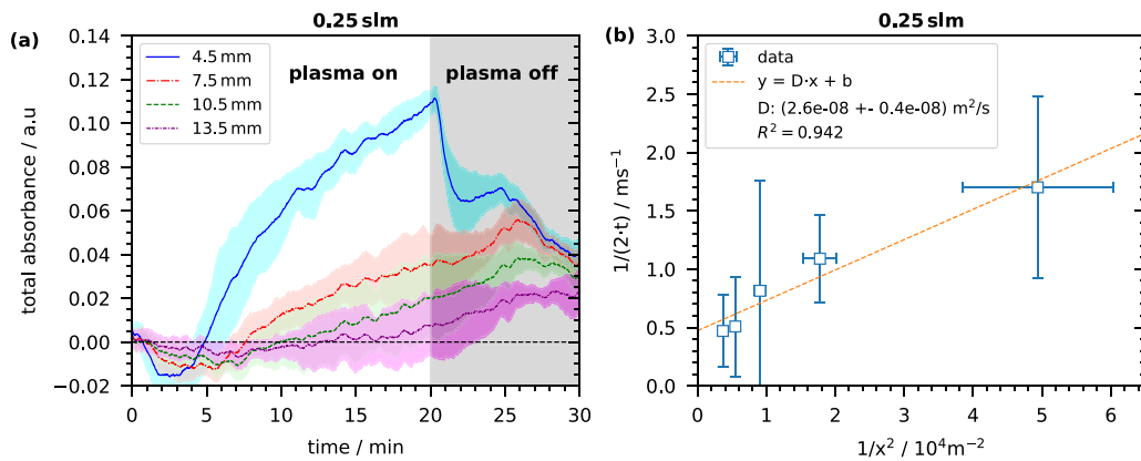
Figure 4. (a) Total absorbance from 237 nm to 271 nm of plasma-generated \text{H}_2\text{O}_2 over treatment time for a gas flow rate of 0.25 slm at various depths within the liquid. Mean (lines) and standard deviation (shaded area) of three measurements are shown. Individual measurements are shown in SI. Plasma was operated at 6 W and a humidity of 6400 ppm. (b) Plot of 1/(2t) as a function of 1/x^2 to determine the effective diffusion coefficient, which is given by the slope of the linear fit.
