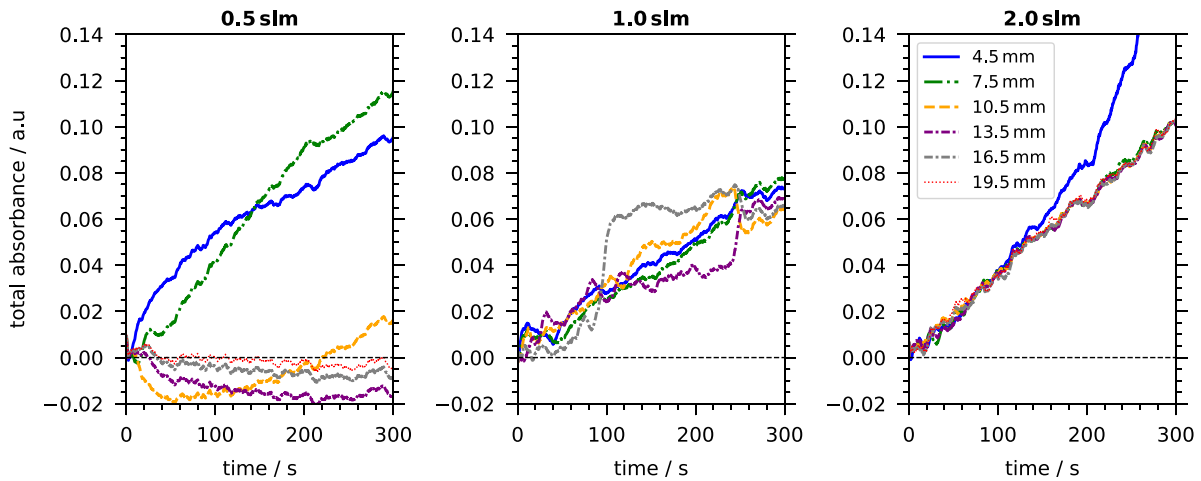
Figure 3. Total absorbance from 237 nm to 271 nm of plasma-generated \text{H}_2\text{O}_2 over treatment time for gas flow rates of 0.5 slm, 1 slm and 2 slm at various depths within the liquid. Plasma was operated at 6 W and a humidity of 6400 ppm. Legend is true for all. Please note that the depth of 19.5 mm could not be evaluated for the case of 1 slm due to disturbances.
