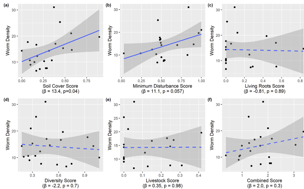
Figure 4. Application of the H3 scoring system to test the impact of implementing different practice combinations on earthworm density (average worms/site). Individual practice scores for (a) soil cover and (b) minimizing disturbance have a larger impact on earthworm density, than individual scores for (c) maintaining living roots, (d) increase diversity and (e) integrating livestock. Overall scores aggregated across principles (f) explain variation in earthworm density less well than some of the individual principle scores. Dashed lines indicate non-significant trends. See electronic supplementary material for more detail on model outputs.
