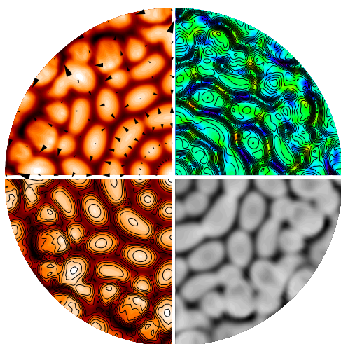
(e) Q = 700 , \Gamma = 6 , and \max(\sqrt{Q}|\bar{B}|) = 67.07 at time 1443.92
