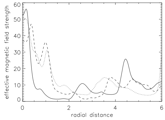
(b) Radial profile of three instances from (a). The solid line is at time 1529.45, the dotted line at 1011.42 and the broken line at 491.46.
