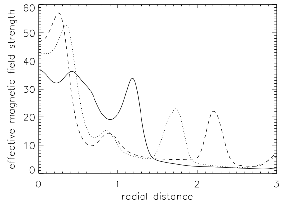
(b) Radial profile of three instances from (a). The solid line is at time 1761.09, the dotted line at 1179.1 and the broken line at 592.86.
