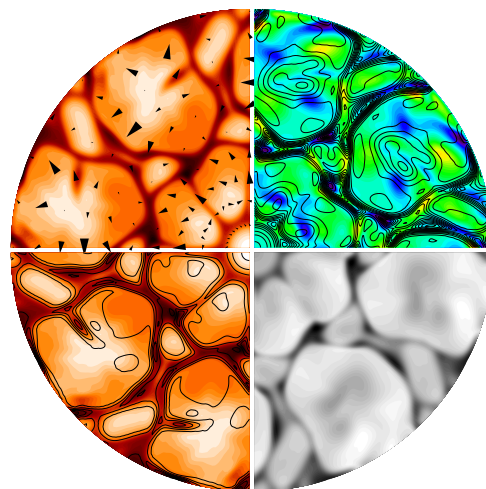
(d) Q = 250 , \Gamma = 6 , and \max(\sqrt{Q}|\bar{B}|) = 87.15 at time 2679.2
