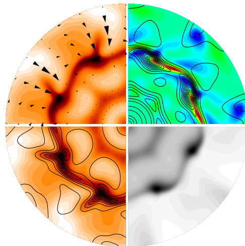
(b) Q = 250 , \Gamma = 3 , and \max(\sqrt{Q}|\bar{B}|) = 101.25 at time 5519.43
