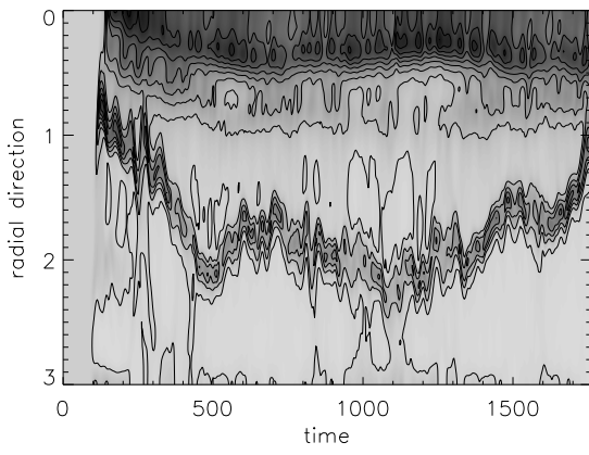
(a) Q = 32 with \max(\sqrt{Q}|\bar{B}|) = 63.09
