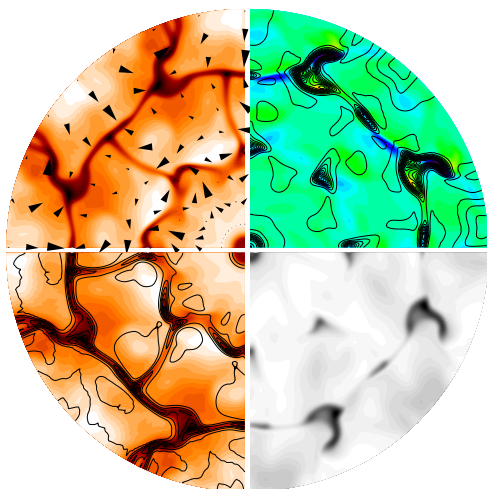
(c) Q = 32 , \Gamma = 6 , and \max(\sqrt{Q}|\bar{B}|) = 101.25 at time 1509.8
