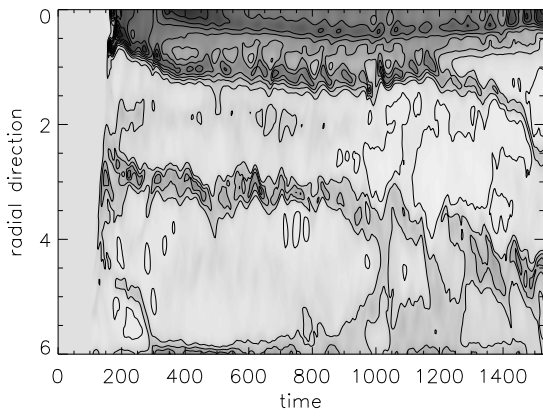
(a) Q = 32 with \max(\sqrt{Q}|\bar{B}|) = 68.38
