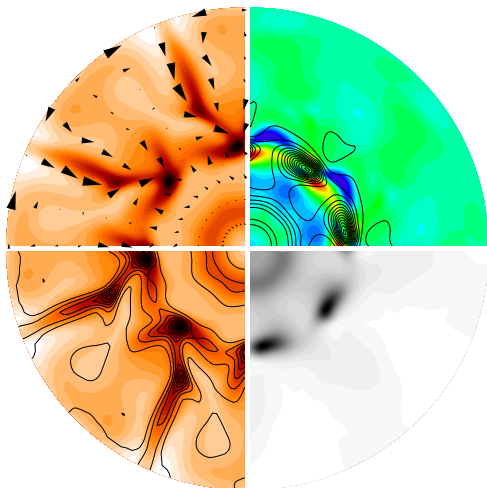
(a) Q = 32 , \Gamma = 3 , and \max(\sqrt{Q}|\bar{B}|) = 101.25 at time 1761.53
