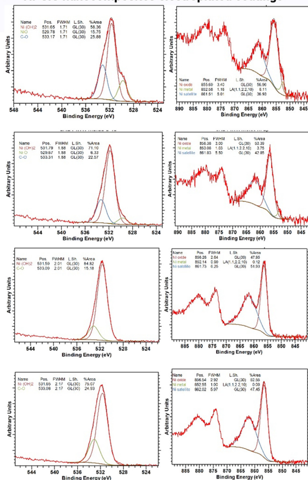
Fig. 3 Characterisation of Ni Watt type and Ni-SiC nanocomposite electroplated coating post aging in various media. (A) TEM analysis of Ni-SiC electroplated aging in artificial sea water (ASW), wastewater (WW), cell culture media (CCM), and 1 mM NaNO 3 . XPS analysis of Ni-Watts type coatings (B) and Ni-SiC (C) nanocomposite coatings in various simulated media showing transformation of Ni in various media. The chemical composition and respective peaks for Ni and O are shown in the graphs.
