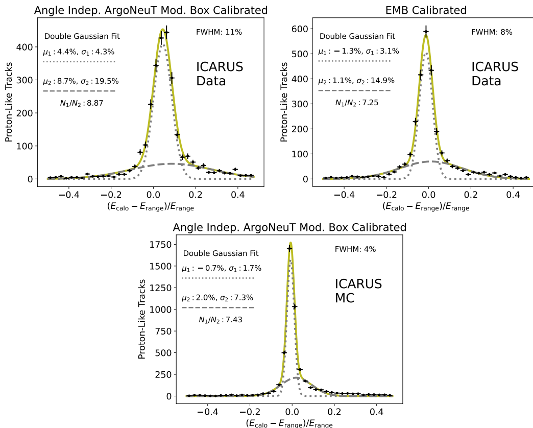
Figure 12. Comparison of calorimetric energy ( E_{\text{calo}} ) and range energy ( E_{\text{range}} ) reconstruction (as defined in section 6.2) for selected protons in ICARUS data (top) and Monte Carlo simulation (bottom). The comparison is made in data for the ArgoNeuT angle-independent modified box-based calibration (top-left) and the EMB-based calibration (top-right). The Monte Carlo simulation applies the ArgoNeuT angle-independent modified box model for both simulating recombination and correcting for it. The data points are fit to a sum of two Gaussian distributions with centers ( \mu_1 , \mu_2 ) and standard deviations ( \sigma_1 , \sigma_2 ). The ratio of the amplitudes of the Gaussian distributions is quoted as N_1/N_2 .
