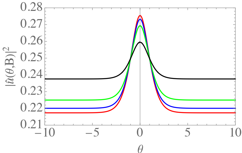
Figure 1: The absolute value squared of the function \hat{u}(\theta, B) := \frac{u(\vartheta, B)}{i + \sinh \theta} with u(\vartheta, B) = \exp \omega(\vartheta, B) evaluated numerically from (28). The colours correspond to different values of B : B = 1 (red), B = 0.7 (blue), B = 0.5 (green) and B = 0.2 (black).
