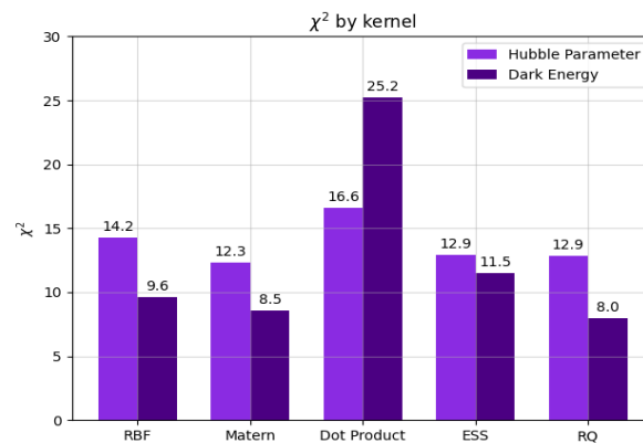
Figure 8. Models with different kernels were produced for both the Hubble Parameter and the Dark Energy functions, and its \chi^2 values were computer. As observed, the optimal covariance function was the Matern for the Hubble Parameter and the Rational Quadratic for the Dark Energy.
