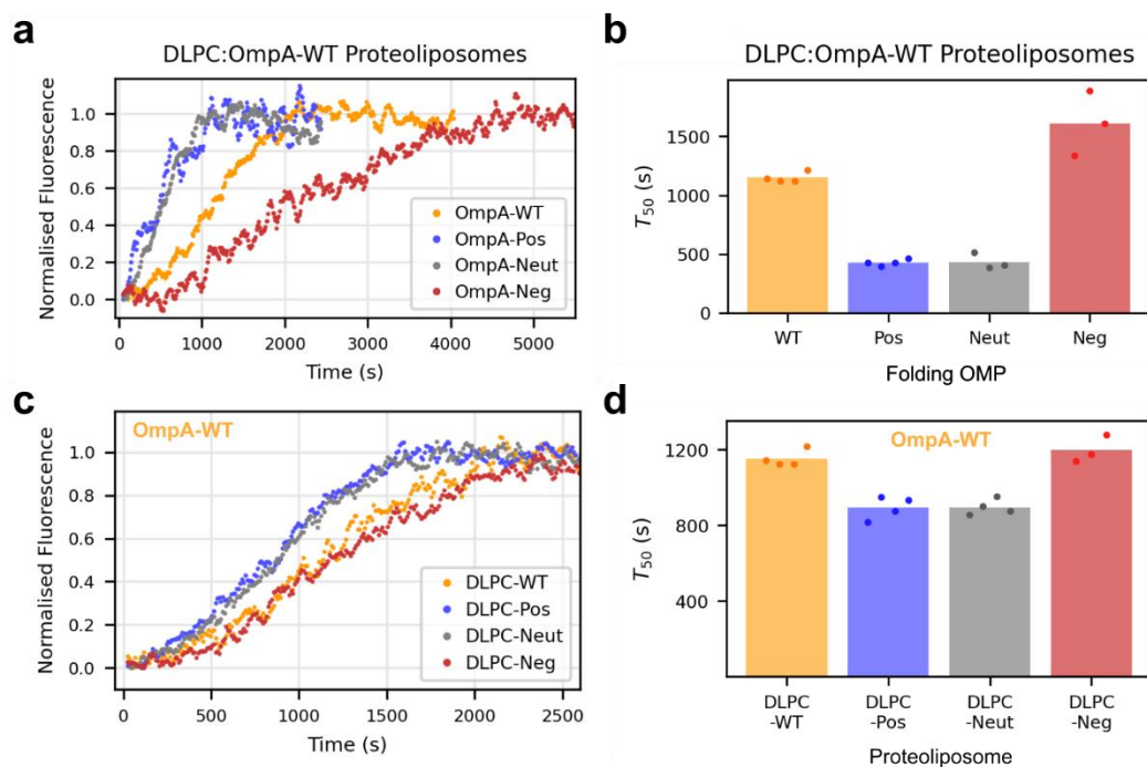
Figure 4: Both OmpA sequence and the charge dipole modulate the folding kinetics. (a) Sample kinetic traces of OmpA variants folding into DLPC:OmpA-WT proteoliposomes and (b) fitted T_{50} values for each curve ( n \geq 3 ). (c) Sample kinetic traces for OmpA-WT folding into proteoliposomes with different dipoles and (d) fitted T_{50} values for each curve ( n \geq 3 ). Data for DLPC-WT are reproduced from (b) for ease of comparison. (LPR of all proteoliposome substrates \sim 320:1 ).
