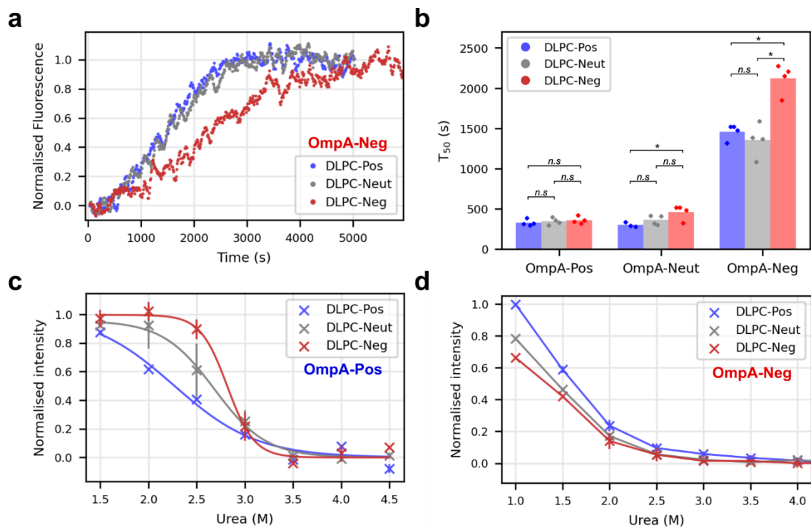
Figure 5: Electrostatic matching between folding OMP and proteoliposome dipole. (a) Sample kinetic traces of OmpA-Neg folding into differently dipoled proteoliposomes as indicated in the key. (b) Comparison of folding T_{50} s for OmpA-Pos, OmpA-Neut and OmpA-Neg into differently dipoled proteoliposomes. P-values were determined by permutation testing (* : p = 0.028 ) ( n \geq 3 ). (c) Urea dependence of OmpA-Pos folding into differently dipoled proteoliposomes ( n = 2 , error bars show data range). Curves are fitted to the average data (bold symbols). (P-values: DLPC-Pos/DLPC-Neg: 0.014, DLPC-Pos/DLPC-Neut: 0.040, DLPC-Neg/DLPC-Neut: 0.135). (d) Urea dependence of OmpA-Neg folding into differently dipoled proteoliposomes ( n = 2 , error bars show data range, n=1 for values at 1 M urea). Lines join the points and are to guide the eye only. (P-values: DLPC-Pos/DLPC-Neg: 0.010, DLPC-Pos/DLPC-Neut: 0.010, DLPC-Neg/DLPC-Neut: 0.042). (LPR of proteoliposome substrates in all panels \sim 320:1 ).
