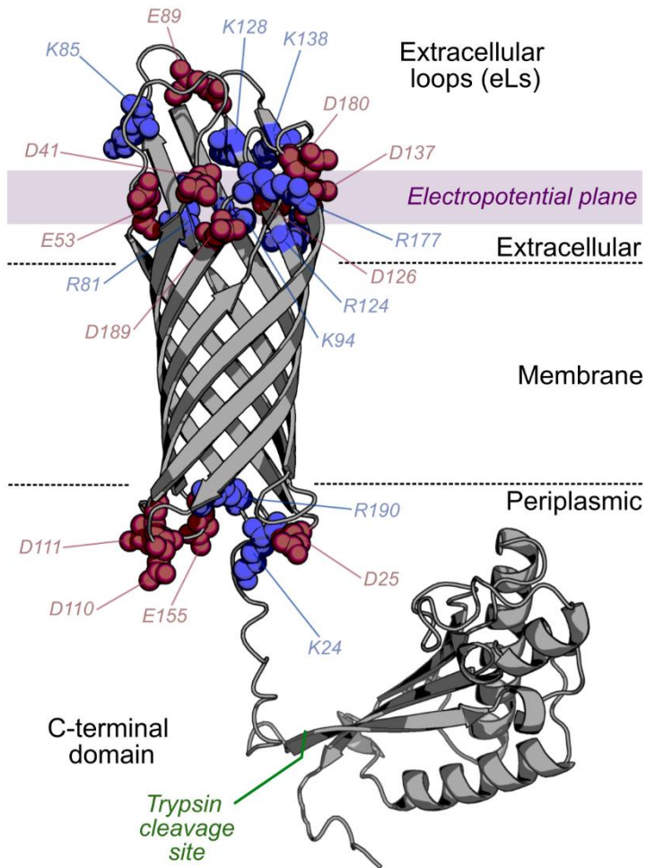
Figure 1: Structural overview and charged residues of OmpA. Full length OmpA has a transmembrane \beta -barrel and a natively periplasmic soluble domain joined by a flexible linker. All solvent accessible charged residues (following trypsin cleavage, site marked in green) are shown as spheres and labelled (red: negative, blue: positive). The electropotential plane indicates the approximate region used to calculate the electrostatic potential shown in Figure 2a . OmpA-Neg neutralises all labelled positive extracellular residues (R81S, K85T, K94S, R124S, K128G, K134S and R177S), OmpA-Pos neutralises all labelled negative extracellular residues (D41S, E53N, E89V, D126S, D137S, D180S and D189S). OmpA-Neut neutralises all extracellular positive and negative residues by combining the OmpA-Pos/-Neg mutations. (OmpA modelled from PDBs 1G90 1 (transmembrane) and 2MQE 2 (C-terminal domain)).
