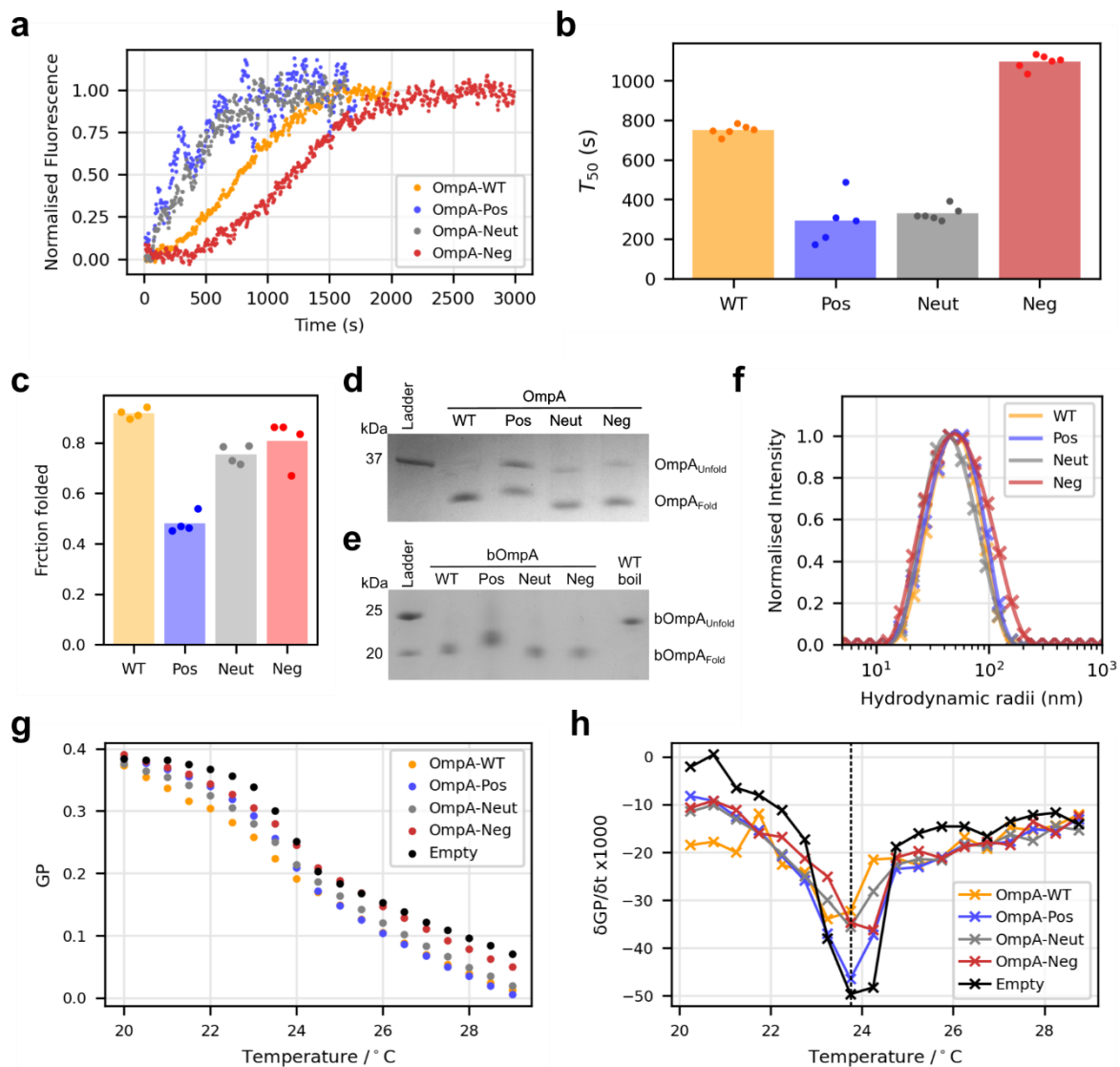
Figure 3: OmpA folding into DLPC and proteoliposome validation. (a) Example folding kinetics for the four OmpA variants inserting into empty DLPC liposomes and (b) fitted half-times ( T_{50} ) for each curve ( n \geq 5 ). (c) Fraction of each OmpA-variant folded into DLPC liposomes at an LPR of 320:1 (mol/mol). (d) By matching the LPR to the yield of each folded protein, proteoliposomes with similar concentrations of each natively folded OmpA variant can be generated. (Original image in Supplementary Fig. 3 ). (e) After cleavage of the C-terminal soluble domain with trypsin and purification, proteoliposomes with a similar LPR containing only the (folded) barrel domain of OmpA are recovered. (Original image in Supplementary Fig. 4 ). (f) DLS of the final proteoliposomes used for folding assays. (g) The GP (generalised polarisation) ratio of laurdan fluorescence at 440 nm and 490 nm against temperature for DMPC liposomes containing each OmpA variant. (h) The first derivative of the GP indicates only small changes in the lipid T_m (curve minima) in the presence of each protein compared to empty liposomes (dashed line).
