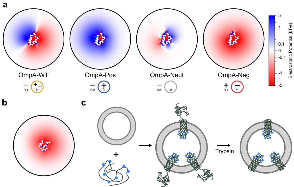
Figure 2: Modelling protein-induced charge-asymmetric liposomes. (a) Modelled electrostatic potential above the membrane plane around the extracellular loops of OmpA variants in DLPC membranes. The direction of the dipole generated from proteoliposomes of each variant is shown beneath each potential map. (b) Modelled electrostatic potential below the membrane plane around the intracellular turns of OmpA. (In (a) and (b) white dots are in-view C \alpha ; circular area is equivalent to the 320:1 (mol/mol) experimental lipid:protein ratio used, ~1 nm solvent slab analysed parallel to the membrane plane). (c) Experimental approach to generate protein-induced charge dipoles over the membrane: OmpA variants are unidirectionally inserted into pre-formed liposomes to a defined concentration, and then the soluble C-terminal domain is cleaved off using trypsin and the resultant proteoliposomes purified. The charge on the extracellular loops (here inside the liposomes when OmpA is folded) are altered by mutation (OmpA-Pos is shown here as an example, with blue positively charged symbols showing the seven positively charged residues in its extracellular loops).
