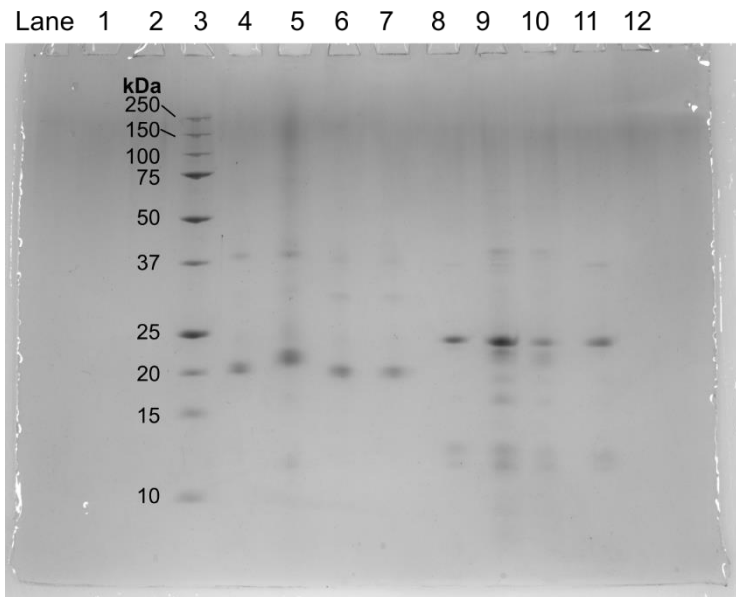
Supplementary Figure 4: Original SDS PAGE gel image for Figure 3e. Lane 1-2: empty, 3: ladder, 4: DLPC + bOmpA-WT, 5: DLPC + bOmpA-Pos, 6: DLPC + bOmpA-Neut, 7: DLPC + bOmpA-Neg, 8: DLPC + bOmpA-WT boiled, 9: DLPC + bOmpA-Pos boiled, 10: DLPC + bOmpA-Neut boiled, 11: DLPC + bOmpA-Neg boiled, 12: empty. The lower molecular weight bands in the lanes of boiled samples indicate some of the bOmpA is also cleaved, however, as the same sample migrates as a single-band in the unboiled lanes, a single intact barrel structure must be retained, thus the generated dipoles should not be affected by this population.
