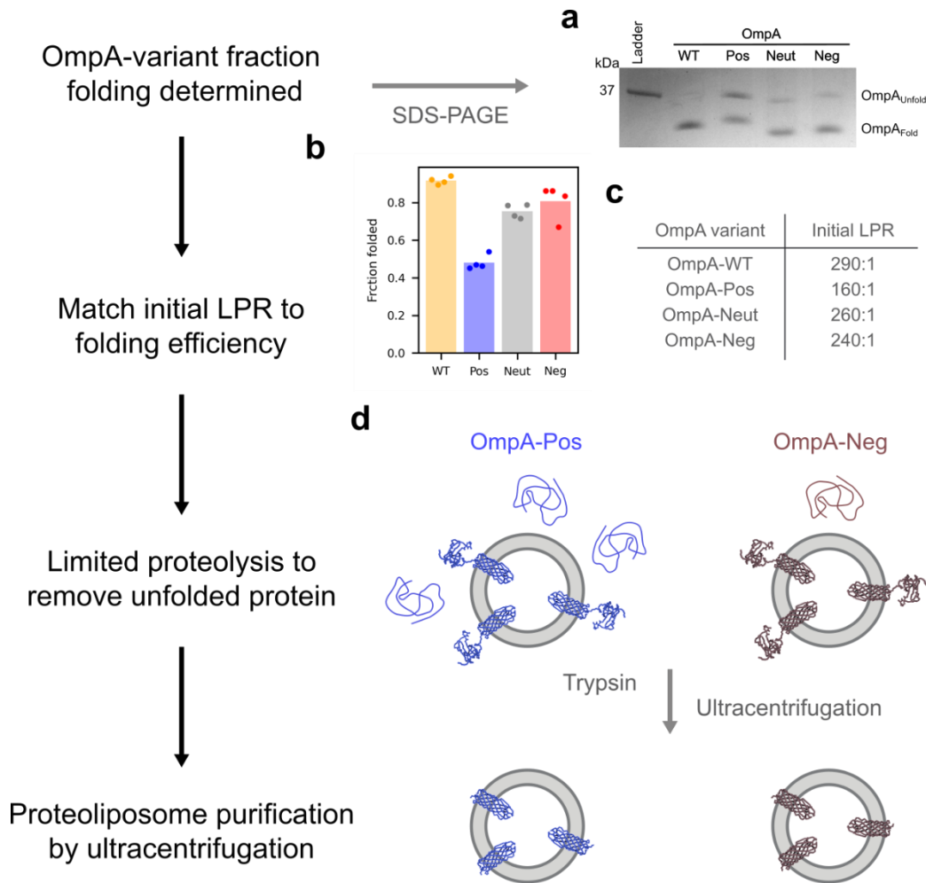
Supplementary Figure 2: Method to generate LPR matched proteoliposomes with OmpA charge variants. Initially the folding efficiency of each OmpA variant was assessed by cold SDS-PAGE (a), which enabled the fraction folded, membrane inserted protein to be determined (b). Guided by the fraction folded, the initial LPR was calculated such that the final, folded OmpA LPR should be 320:1 (c). Following folding, different amounts of unfolded protein remained in solution (d), which were then cleaved, along with OmpA's C-terminal domain, using trypsin. The LPR matched proteoliposomes were then purified via ultracentrifugation and validated (see Figure 3).
