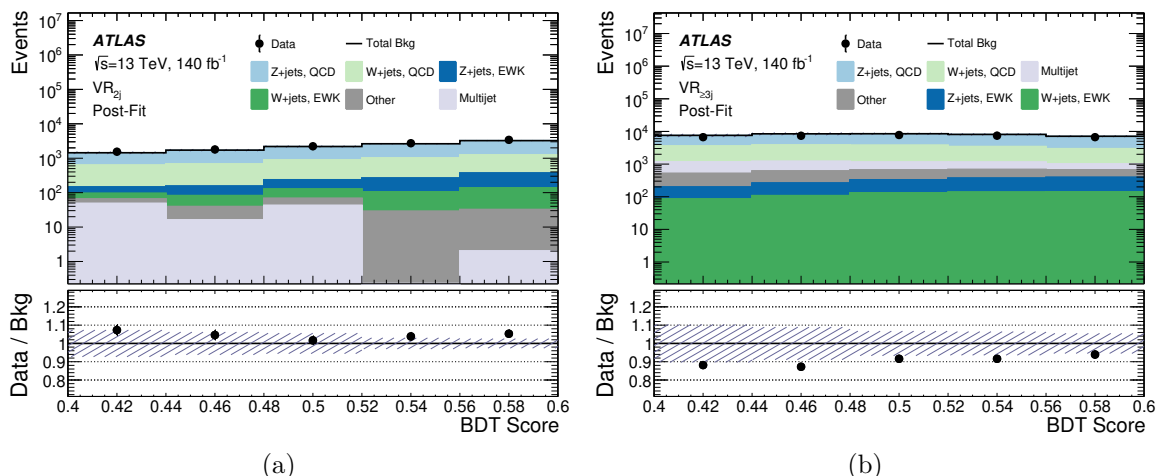
Figure 6. Observed and predicted background distributions of the BDT score in (a) VR-0L 2j and (b) VR-0L ≥3j low-BDT validation regions, using data-driven estimates for the multijet background. The ‘Other’ category contains rare backgrounds from diboson, triboson and top-quark production processes. The hatched band represents the post-fit experimental, theoretical, and statistical uncertainties in the total background. The bottom panel of each plot shows the ratio between the data and the post-fit background prediction.
