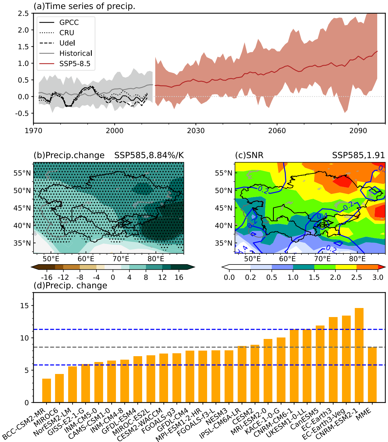
Figure 1. (a) Time series of 5-year running mean winter Central Asian precipitation (WCAP) anomalies (units: mm day -1 ), relative to the present-day average (1970–1999). Historical (gray) and SSP5–8.5 (red) simulations are shown for the minimum and maximum across 25 models (shading), and the ensemble mean (solid lines). The black solid and dash lines are the three observational series (details in Data). (b) Spatial changes in WCAP (units: % K -1 ). The dots denote regions where at least 80% of the models agree on the sign of change. (c) The inter-model SNR (shading) and standard deviation (STD) (contour) of projected WCAP changes. (d) Changes in area-weighted regional mean WCAP (units: % K -1 ) of each model and the ensemble mean. The gray and blue lines indicate the ensemble mean and one STD. The number at upper right in panels (b, c) is the averaged value over CA.
