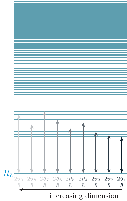
Figure 3. Illustration of the spectrum of the Bochner Laplacian \Delta_{\hbar} = \nabla_{\hbar}^* \nabla_{\hbar} for a symplectic vector space with 18 dimensions ( N=9 ) and diagonal metric components \vartheta_i . The Hilbert space \mathcal{H}_{\hbar} is constructed from the section (66) corresponding to the lowest spectral value (cyan) is the solution.
