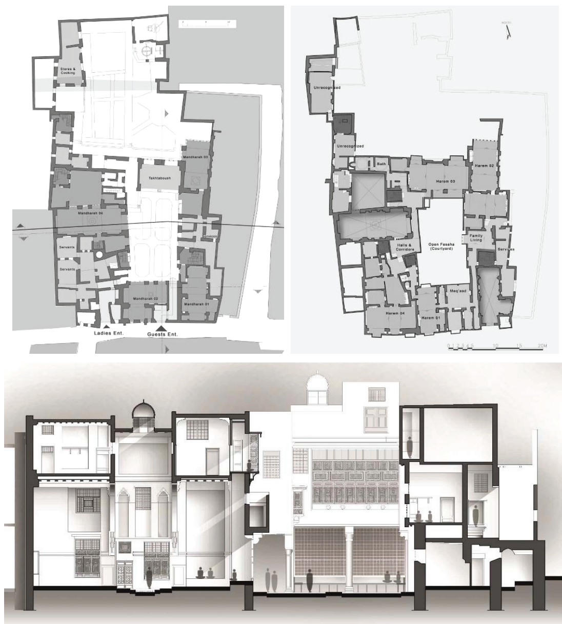
Fig. 5 Bayt al-Suhamy's Floor plans and a section showing the ground floor public sphere.
