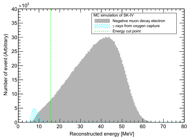
FIG. 17. The reconstructed energy distribution for \gamma -rays from oxygen capture (light-blue right slanting line histogram) as well as that of negative muon decay electron (gray filled histogram), obtained from the MC simulation after applying the selection cuts listed in Table X. The vertical green dashed line shows the optimized cut value used in the analysis.
