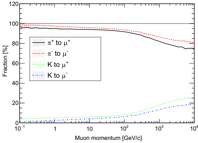
FIG. 1. The fraction of parent particles that produce cosmic-ray muons at the Kamioka site, based on the Honda flux simulation [23]. The fraction is calculated by integrating over the zenith angle. The solid black, dashed red, dotted green, and blue dashed-dotted lines show the fraction of positive pion to positive muon, negative pion to negative muon, kaon to positive muon, and kaon to negative muon, respectively.
