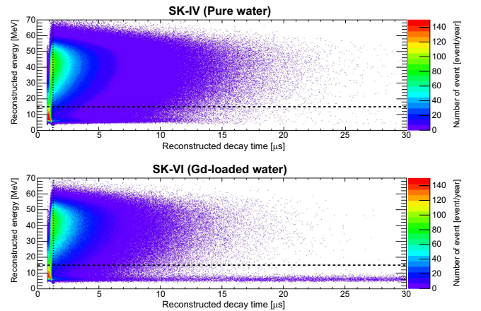
FIG. 29. The time difference between the stopping muon and the reconstructed events in the SK-IV (top) and -VI (bottom) data sample. In the SK-VI data sample, 8 MeV \gamma -rays originating from the neutron capture by gadolinium in water are observed after tagging the decay electron.
