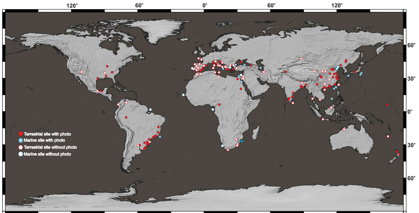
Fig. 4. Biogeography of Chomotriletes s.l. in Plio-Pleistocene and Holocene records. The distribution is based on a selection of the more than 300 compiled occurrences in order to show a maximum distribution. The data underlying the map are presented in Supplementary Table S2.
