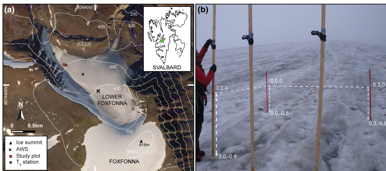
FIGURE 1 (a) Map detailing Lower Foxfonna's setting and topography, and the locations of the 9 m 2 observation plot with a time lapse camera array, the automatic weather station (AWS), and the TinyTag air temperature stations during 2011. The background orthophoto from 2006 was made available by Store Norske Spitsbergen Kulkompani AS. Foxfonna's location in central west Svalbard is shown in the inset. (b) Image of the observation plot, looking up-glacier, illustrating the convergent camera set-up and reference markers with approximate scales and distances shown for the arbitrary coordinate system employed (photograph credit: Arwyn Edwards) [Color figure can be viewed at wileyonlinelibrary.com ]
