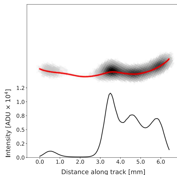
Fig. 21. Reconstructed track for the 5 keV Migdal electron event shown in Fig. 20 (right), after applying deconvolution and track-finding algorithms to the camera image; the resultant track ridge is shown in red. The plot in the lower part of the frame shows the intensity integrated transversally along the tracks (rather than a straight projection) and is meant to illustrate the very different energy loss rates along NR and ER tracks.
