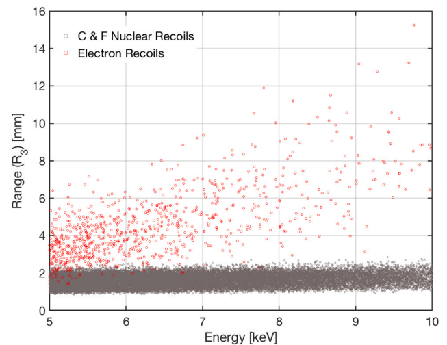
Fig. 22. 3D range as a function of reconstructed energy (keV _{ee} ), showing separation of low-energy electrons (wide band) from carbon and fluorine recoils (narrow band) in \text{CF}_4 at 50 Torr.
