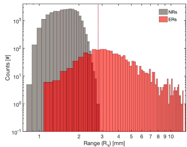
Fig. 23. Distribution of 3D range in the 5–10 keV _{ee} ROI shown in Fig. 22. A cut at R_3 = 2.80 mm gives a leakage of 1 background events per million NR tracks, with a corresponding acceptance of ER signals of 87% (see text for details).
